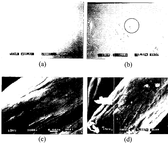
Figure 8. SEM photographs of IEC and IXF. (a) before adsorption (IEC), (b) after adsorption (IEC), (c) before adsorption (IXF), and (d) after adsorption (IXF).
