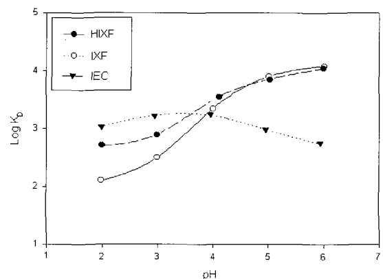
Figure 2. Distribution coefficient of NO 3 - ion on different pH of IEC, IXF and HIXF ion exchanger.
