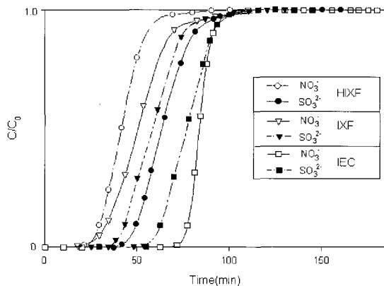
Figure 6. Normalized breakthrough curve for NO_3^- and SO_3^{2-} according to adsorption time.
