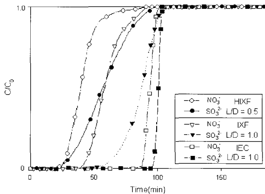
Figure 5. Normalized breakthrough curve for NO_3^- and SO_3^{2-} in mixed solution with time of bed volume.
