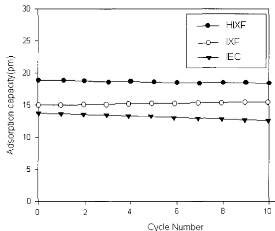
Figure 7. Dependence of the NO_3^- adsorption capacities of ion exchangers with regeneration frequency.
