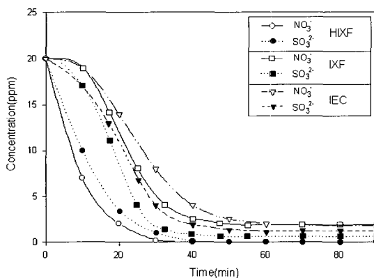
Figure 3. Concentration(ppm) of NO 3 - and SO 3 2- in mixed solution with time by batch process.
