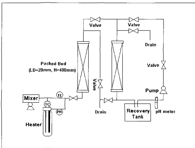
Figure 1. Schematic diagram of adsorption experiment apparatus.
