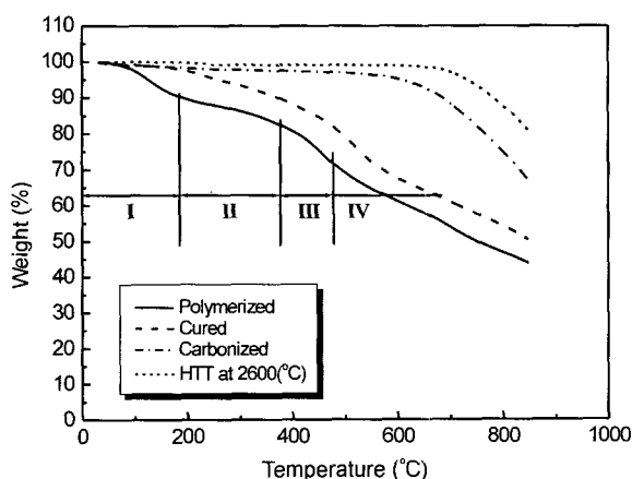
Figure 1. TGA analysis of samples obtained from the consecutive heat treatment processes to make glass-like carbon from furan resin.
