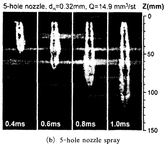
Fig. 5 Mie scattering images of 3-hole and 5-hole nozzles spray with time from SOI
