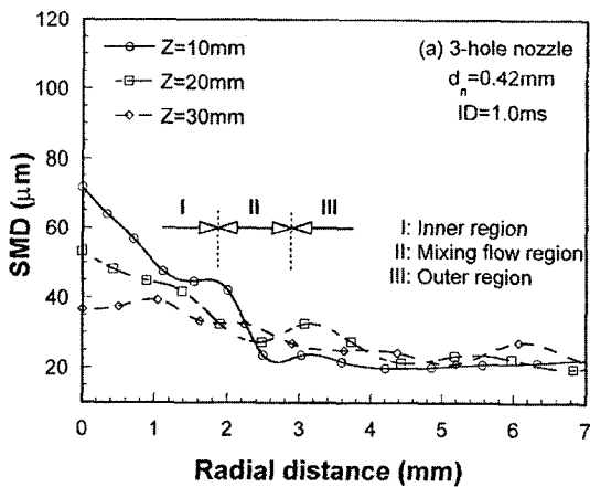
(a) 3-hole nozzle ( d_n=0.42 mm, ID=1.1 ms)
