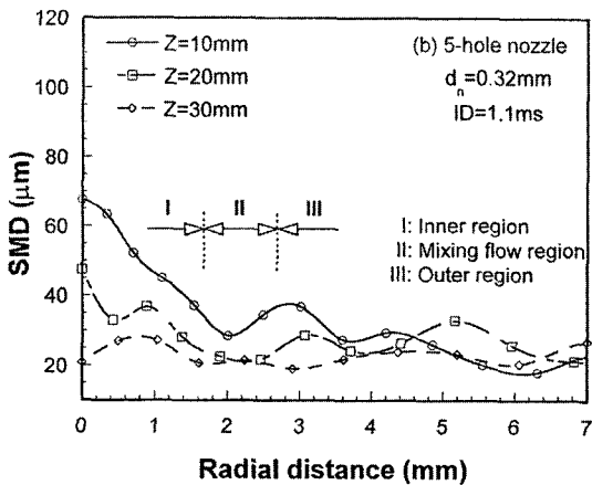
(b) 5-hole nozzle ( d_n=0.32 mm, ID=1.1 ms)
