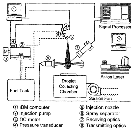
Fig. 1 Schematic diagram of experimental apparatus for droplet size measurement using 2-D PDPA system
