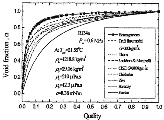
Fig. 9 Variations of the void fraction predicted from various correlations
