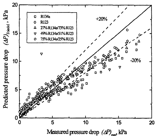
Fig. 10 Comparison between measured data and Friedel correlation
