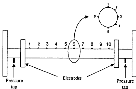
Fig. 2 Test section
