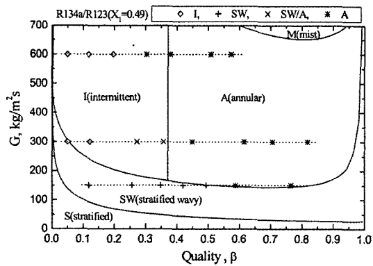
Fig. 4 Flow patterns on the G - \beta map
