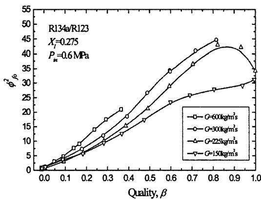
Fig. 6 Variations of the two-phase frictional multipliers against quality
