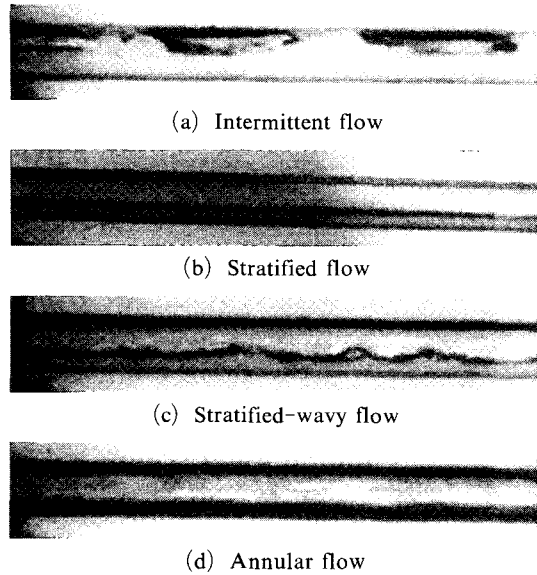
Fig. 3 Typical pictures of flow patterns
