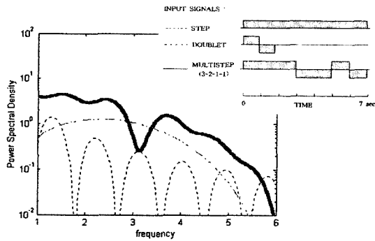
Fig. 1 Frequency domain comparison of various input signals
