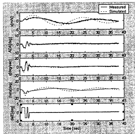
Fig. 8 Flight test data compared with DATCOM modeling (longitudinal)
