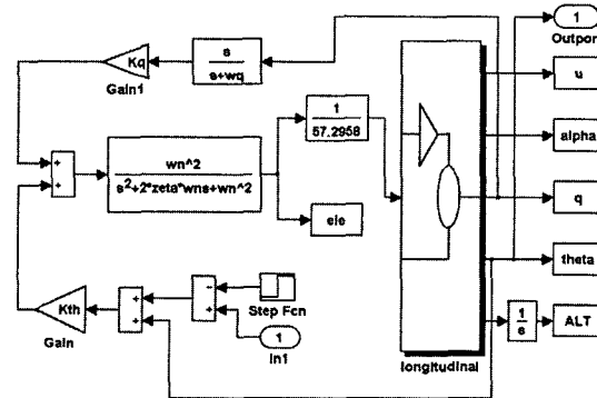
Fig. 2 Pitch loop block diagram
