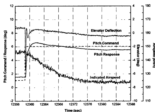
Fig. 3 Closed-loop flight test data
