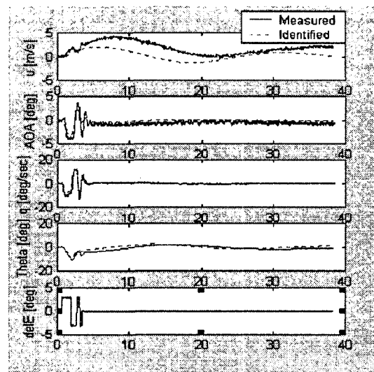
Fig. 10 Longitudinal identification results (open-loop, high speed)
