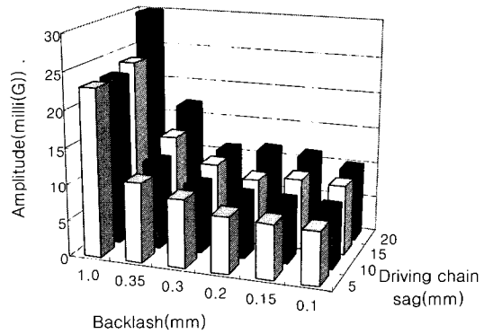
Fig. 9 Vibration levels(3.65 Hz) with respect to driving chain sag and gearbox backlash (test)
