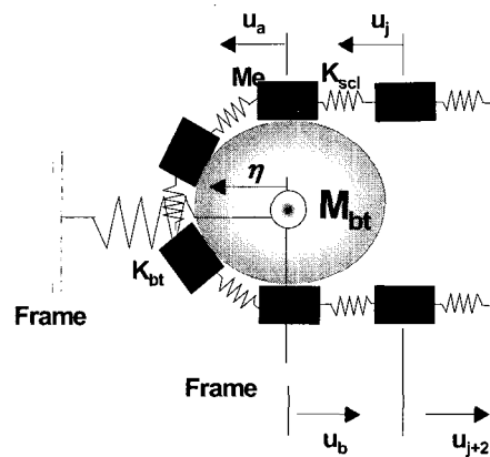
Fig. 5 Schematic vibration model for lower guide
