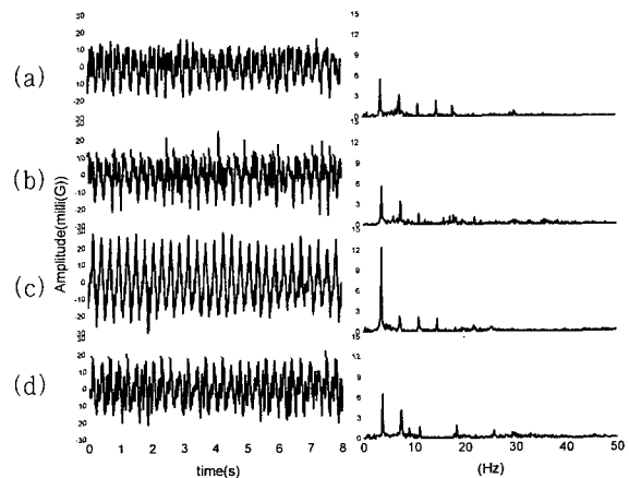
(a) Vibration in up direction(600 N) (b) Vibration in down direction(600 N) (c) Vibration in down direction(1800 N) (d) Vibration in down direction(3000 N)
