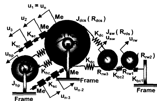
Fig. 4 Schematic vibration model for upper sprocket and driving units
