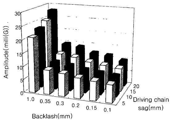
Fig. 8 Vibration levels(3.65 Hz) with respect to driving chain sag and gearbox backlash
