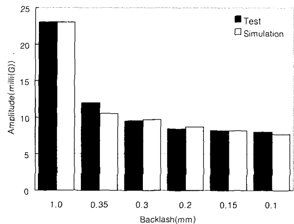
Fig. 7 Comparison of vibration levels(3.65 Hz) with respect to gearbox backlash
