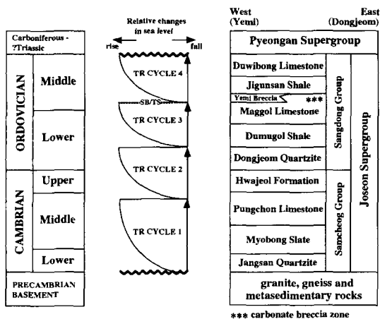
Fig. 2. Lithostratigraphic nomenclature of the Cambro-Ordovician Joseon Supergroup, Backunsan Syncline (Cheong, 1969). TR=transgressive-regressive; SB/TS=sequence boundary/transgressive surface.
