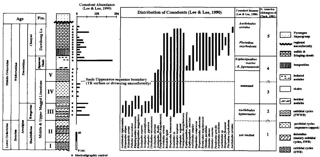
Fig. 5. Composite stratigraphic column and conodont biostratigraphy of the upper Maggol Limestone, the Jigunsan Shale, and the Duwibong Limestone. Conodont biostratigraphy indicates that the Lower to Middle Ordovician chronostratigraphic boundary lies between the unit II and the unit III. Also, the boundary between the unit IV and the unit V may be coincident with the Sauk-Tippeneo sequence boundary of Sloss (1963). Conodont data from Lee and Lee (1990).
