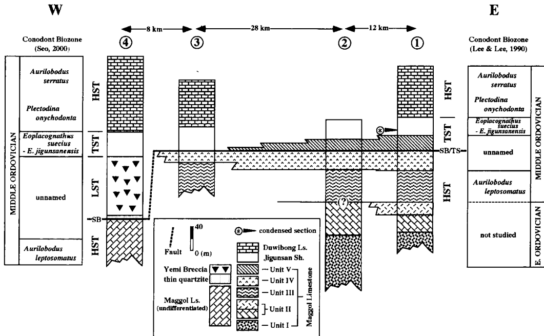
Fig. 8. Schematic sketch illustrating the sequence stratigraphic correlation of the Taebaksan Basin during the Middle Ordovician.
