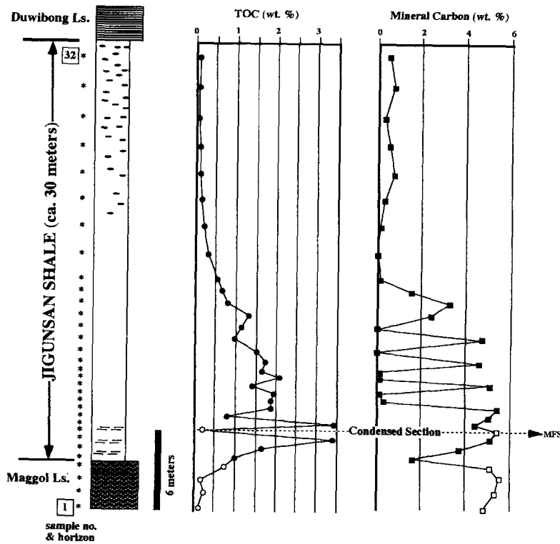
Fig. 7. Vertical variations of total organic carbon and mineral carbon contents of the Jigunsan Shale in the study area.
