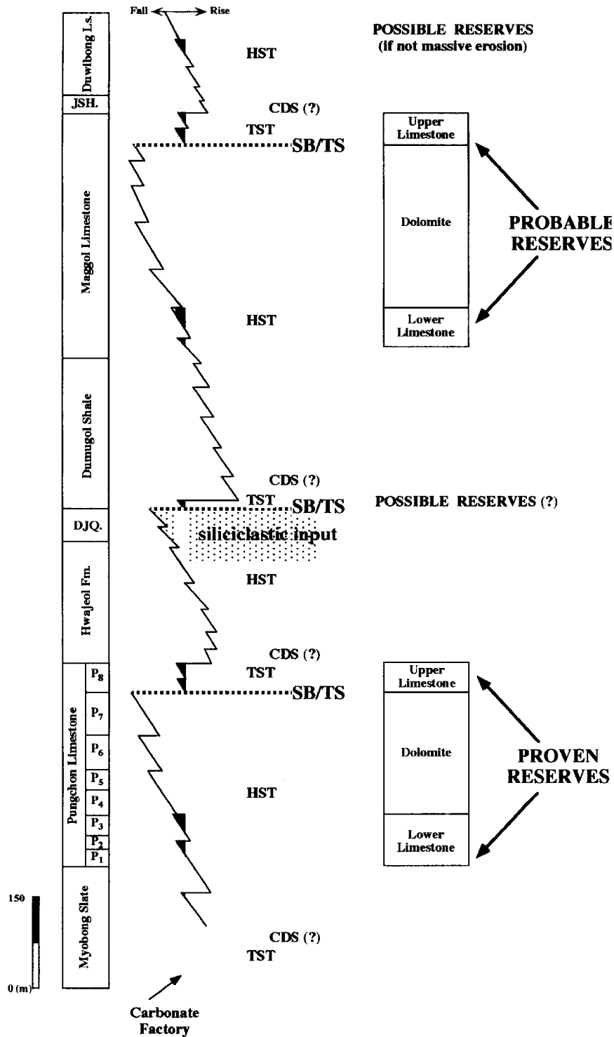
Fig. 10. Vertically-oriented Fischer plot of the Cambro-Ordovician Joseon Supergroup, Dongjeom area, Taebaeksan Basin. Additional limestone reserves in the Taebaeksan Basin probably occur in the Maggol Limestone as well as the lowermost Dumugol Shale and the upper Duwibong Limestone.
