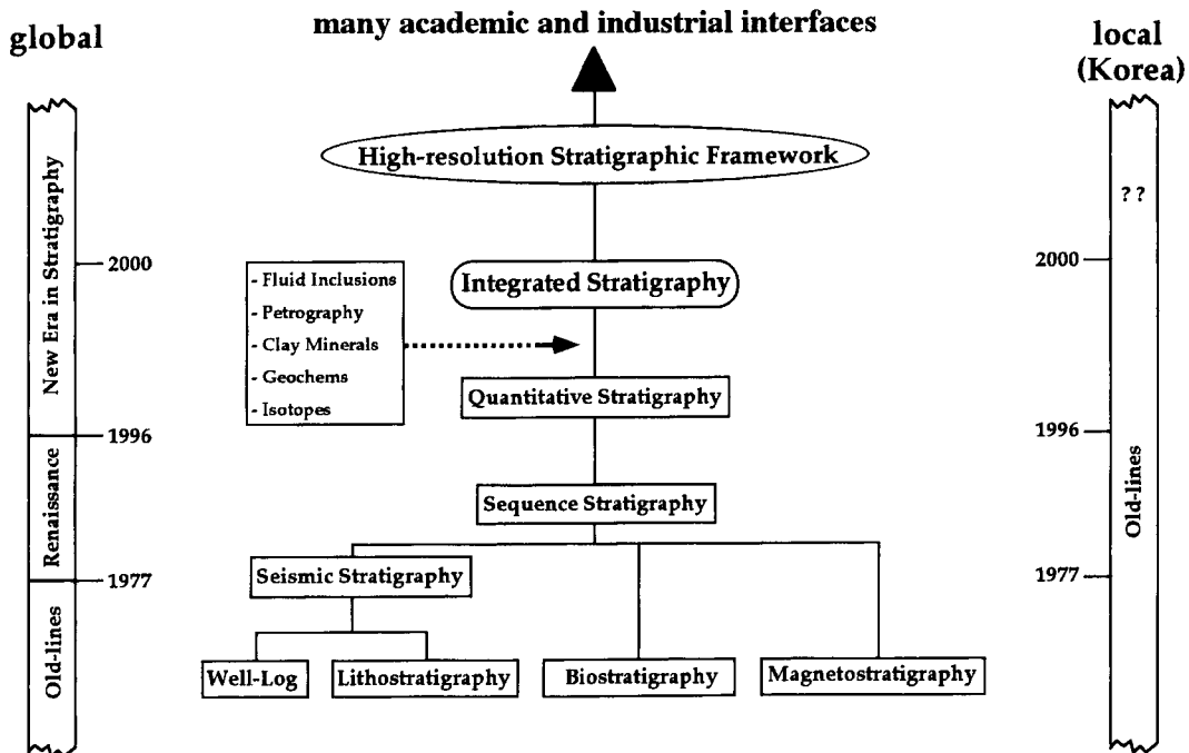
Fig. 12. Diagram showing the developing stage of the integrated stratigraphy technology.
