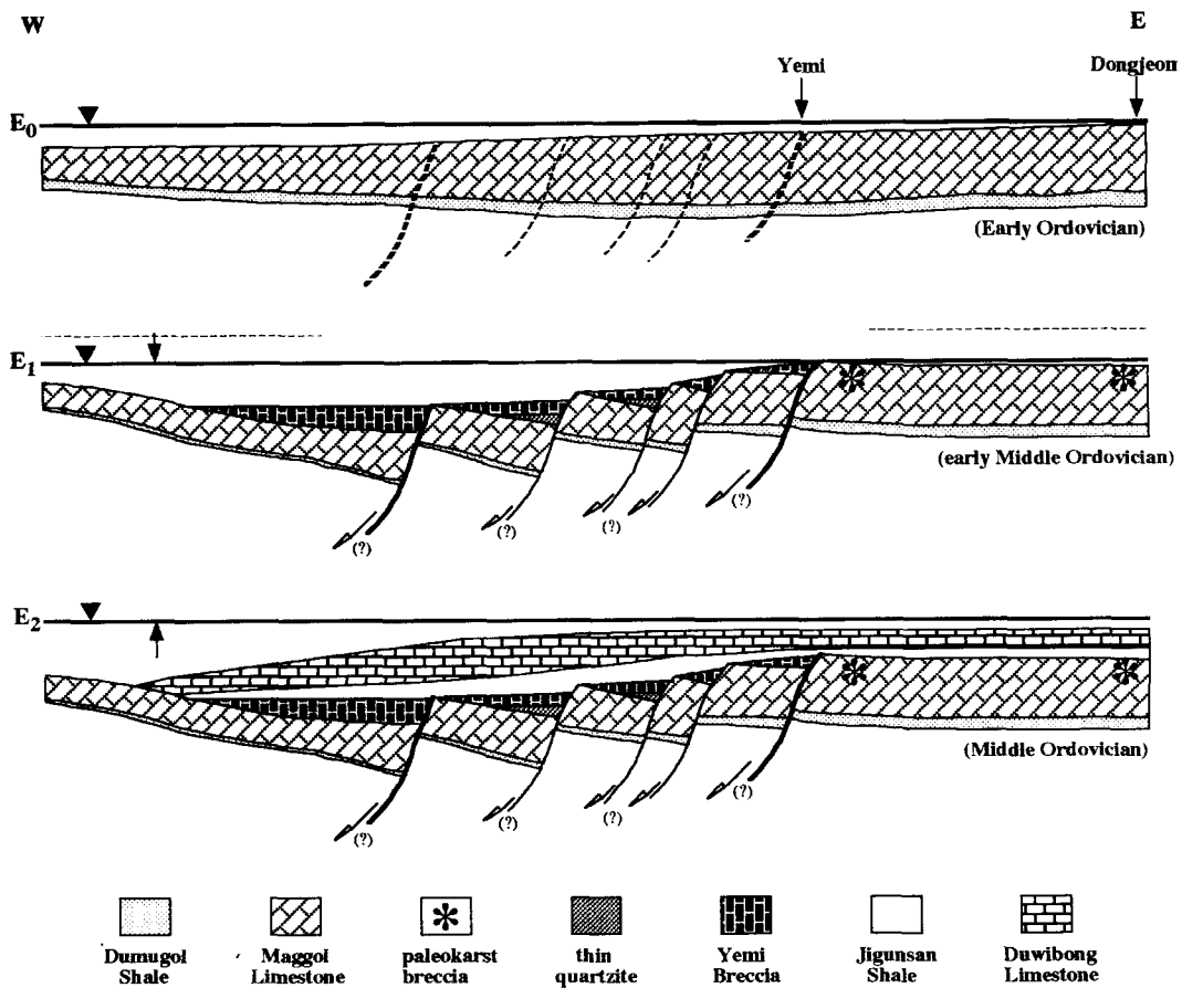
Fig. 11. Schematic sketch illustrating the stratigraphic and tectonic evolution of the Taebaeksan Basin during the Early to Middle Ordovician.
