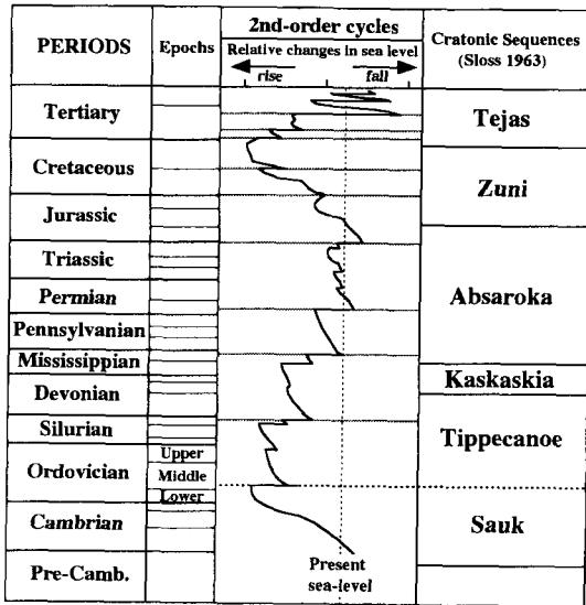
Fig. 6. Temporal correlation of the global sea level change with the subaerial exposure event recognized in the upper Maggol Limestone. The exposure event coincides with the second-order relative sea level drop during the early Middle Ordovician. The second-order global sea level curve from Vail et al. (1977).
