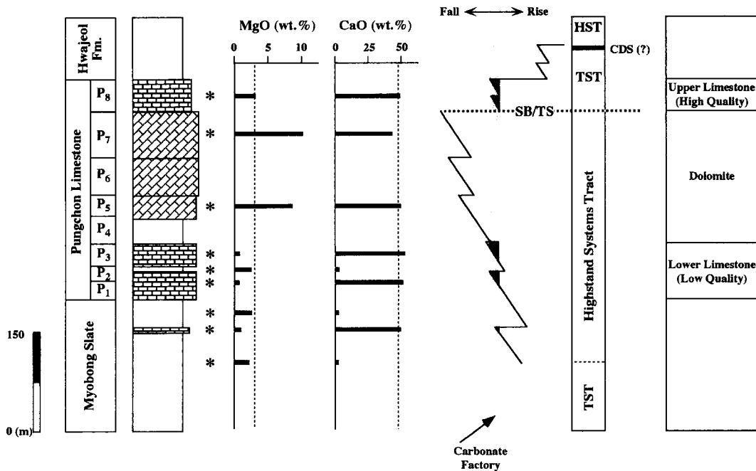
Fig. 9. Generalized lithostratigraphic column and cyclic sedimentation of the Pungchon Limestone. Note the occurrence of high-quality limestones between the sequence boundary and the condensed section as well as the early highstand systems tract. Modified from Yun (1978).
