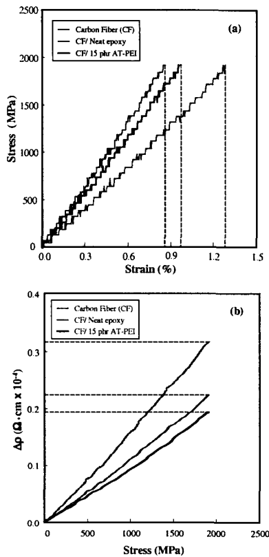
Fig. 11 (a) Stress-strain and (b) change in electrical resistivity-stress curves for carbon fiber/epoxy-AT-PEI composite.
