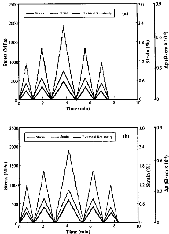
Fig. 10 The change of strain and electrical resistivity for single carbon fiber/epoxy-AT-PEI composite under changable stress.
