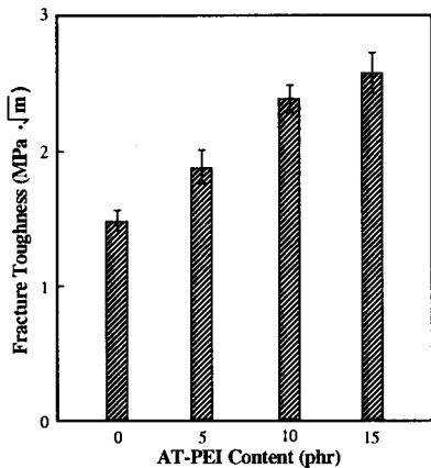
Fig. 5 Fracture toughness of epoxy-AT-PEI matrix with AT-PEI content.
