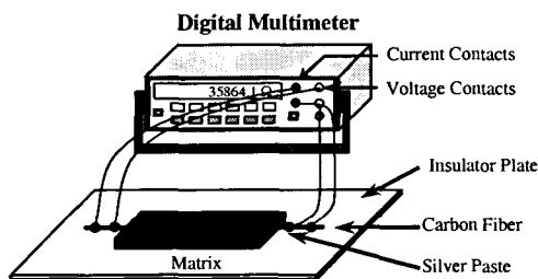
Fig. 1 Schematic diagram for electrical resistance measurement during curing process.
