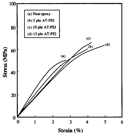
Fig. 4 Stress-strain curves of epoxy-AT-PEI matrix with AT-PEI content.
