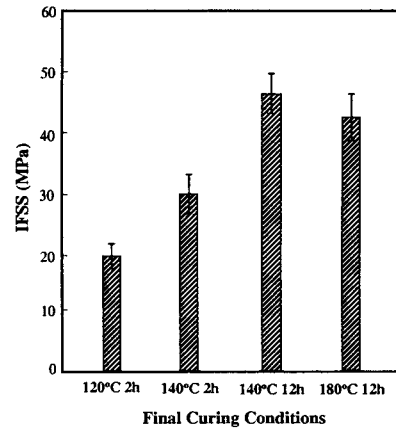
Fig. 6 IFSS of carbon fiber/epoxy-AT-PEI composites with curing conditions.
