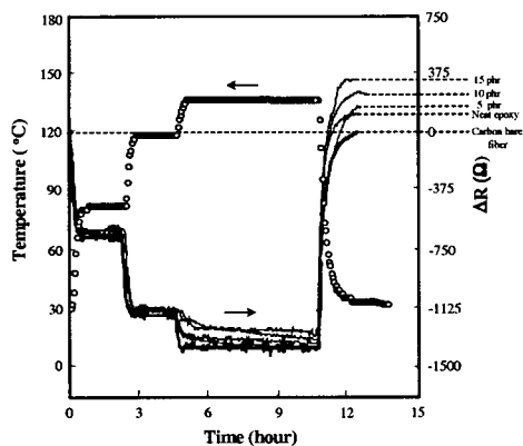
Fig. 9 The changes in electrical resistance for carbon fiber/epoxy-AT-PEI composite.
