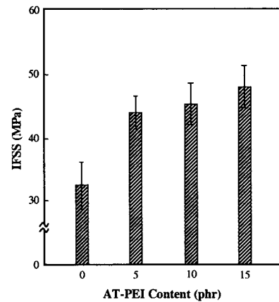
Fig. 7 IFSS of carbon fiber/epoxy-AT-PEI composites with AT-PEI content.
