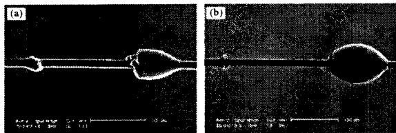
Fig. 8 Typical microfailure modes of carbon fiber/epoxy-AT-PEI composite for (a) neat epoxy and (b) 15 phr AT-PEI.
