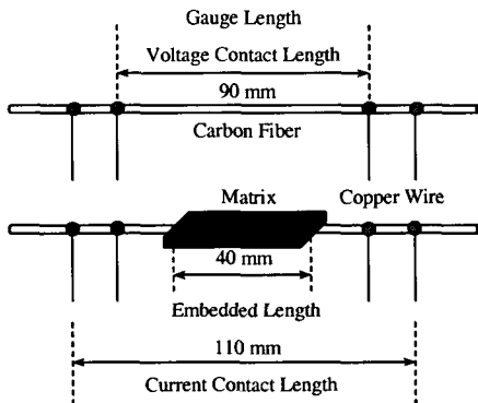
Fig. 2 Schematic diagram for electrical resistance measurement under cyclic loading.
