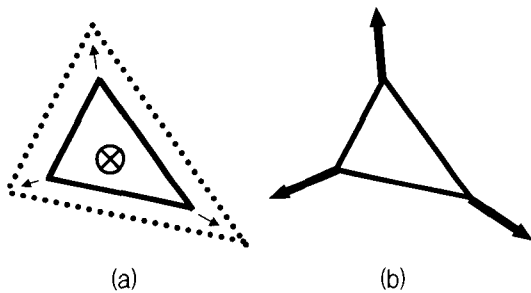
Fig. 6 The center of gravity of the element is considered to be fixed while the magnetostrictive expansion \lambda(B^e) is applied to the nodes. This deformation is represented by a set of mechanical forces
