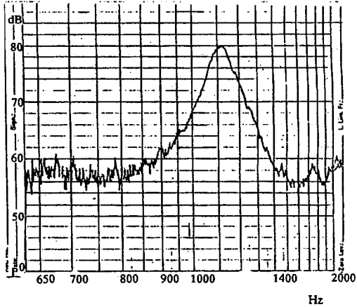
Fig. 5 Narrow-band measurement (without ventilator) of the audible noise of an induction machine at rated load. Motor : 160 kW, 380 V, 50 Hz, 2 p=4, N_1/N_2 = 48/40 (source : (1))
