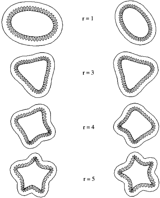
Fig. 4 Various mode shapes of a stator lamination
