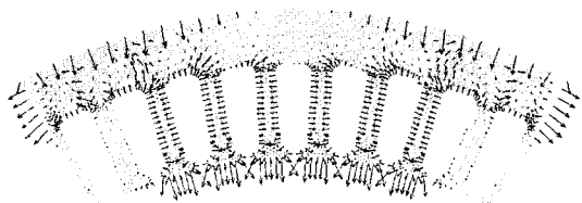
Fig. 10 Comparison between reluctance forces (on the teeth tips) and magnetostriction forces (on the stator surface)
