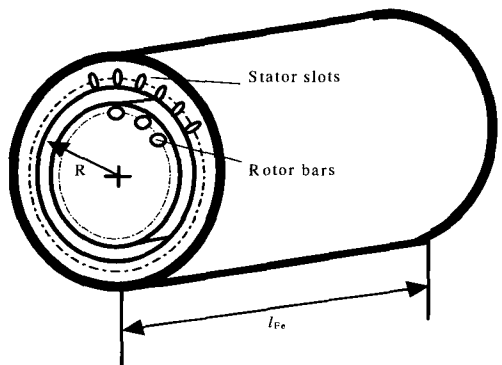
Fig. 3 Construction principle of an induction machine
