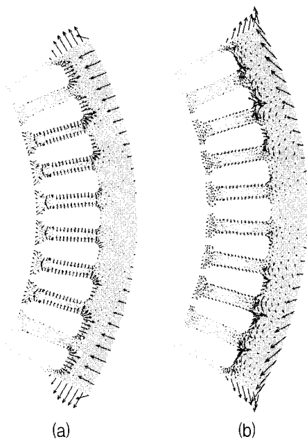
Fig. 9 Magnetostriction forces on stator for (a) isotropic non-oriented 3% SiFe and (b) anisotropic M330-50A
