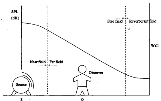
Fig. 2 Noise field definitions
