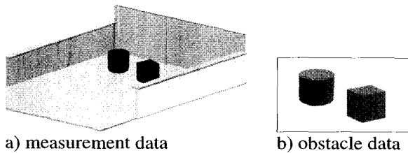
Fig. 4. Obstacle extraction from 3D measurement data using CAD information
