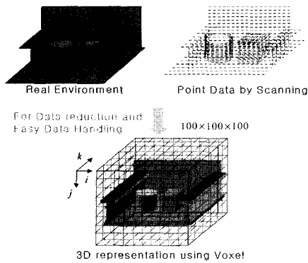
Fig. 2. Voxel representation of measured data.
