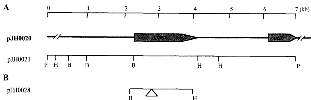
Fig. 1. Physical map of the V. vulnificus pmm gene on the plasmids used in this study.
