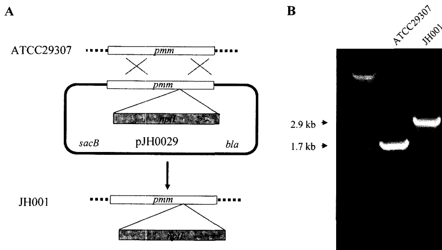
Fig. 3. Allelic exchange procedure and construction of pmm::nptI isogenic mutant.
