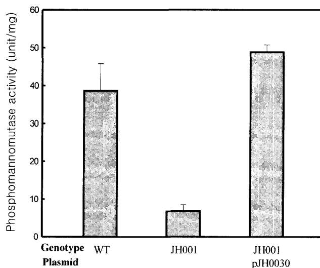
Fig. 4. PMM activities of ATCC29307 and isogenic pmm mutant.
