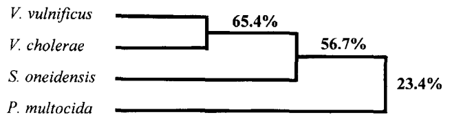
Fig. 2. Amino acid-sequence relatedness of PMMs of V. vulnificus and other bacteria.
