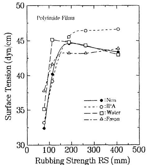
Fig. 4. Surface tension on the PI surface with trifluoromethyl moiety as a function of rubbing strength RS.
