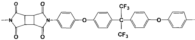
Fig. 1. Molecular structures of the polymers.
