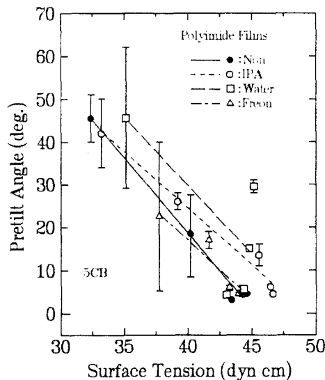
Fig. 5. Pretilt angle of 5CB on the PI surface with trifluoromethyl moiety as a function of surface tension.
