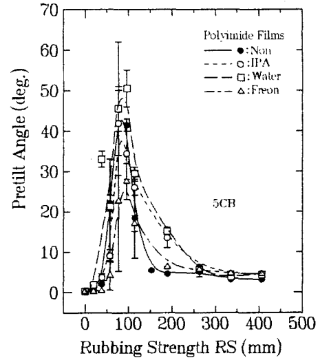
Fig. 3. Pretilt angle of 5CB on the PI surface with trifluoromethyl moiety as a function of rubbing strength RS.
