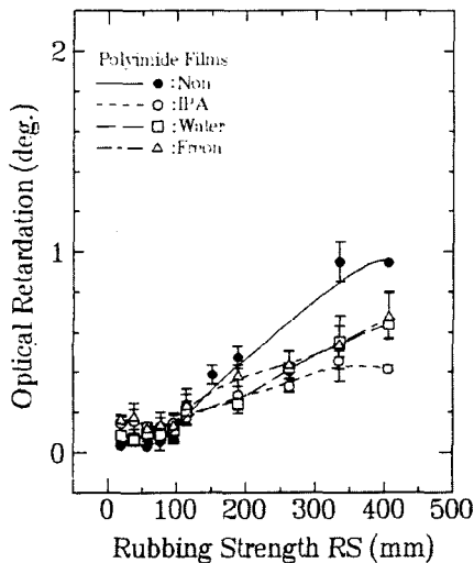
Fig. 2. Induced optical retardation on the PI surface with trifluoromethyl moiety as a function of rubbing strength RS.
