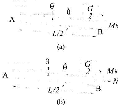
Figure 15. Deformation mechanism of a half of (a) a simply-supported and (b) an axially-constrained beam subjected to a striking mass G at the mid-span.
