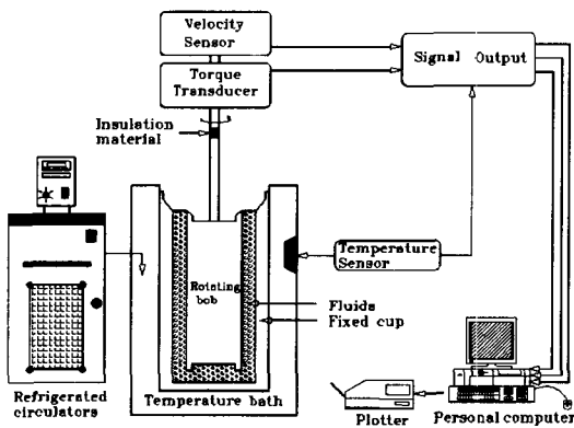
Fig. 8 Schematic of Viscotester (Haake VT500)
