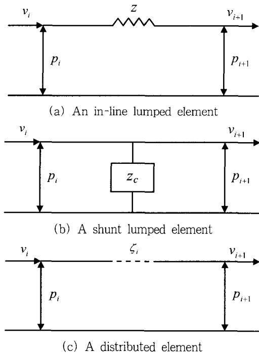
Fig. 1 Representations of acoustic elements in an equivalent electroacoustic circuit (8)
