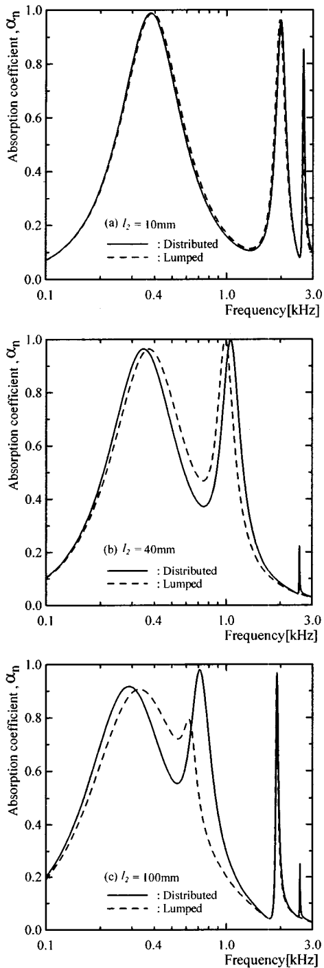
Fig. 5 Comparisons of the absorption coefficients calculated by equivalent electroacoustic circuits based on the distributed element and the lumped parallel element, respectively, for the double layer perforated plate system
