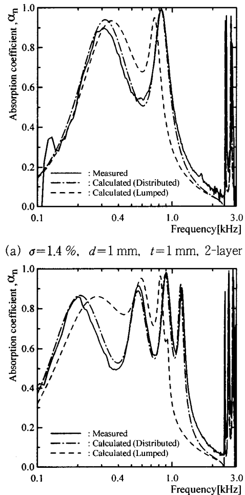
(a) \sigma = 1.4\% , d = 1 mm, t = 1 mm, 2-layer (b) \sigma = 3.14\% , d = 2 mm, t = 1 mm, 4-layer Fig. 6 Comparisons between the measured and the calculated absorption coefficients for the multiple layer perforated plate system
