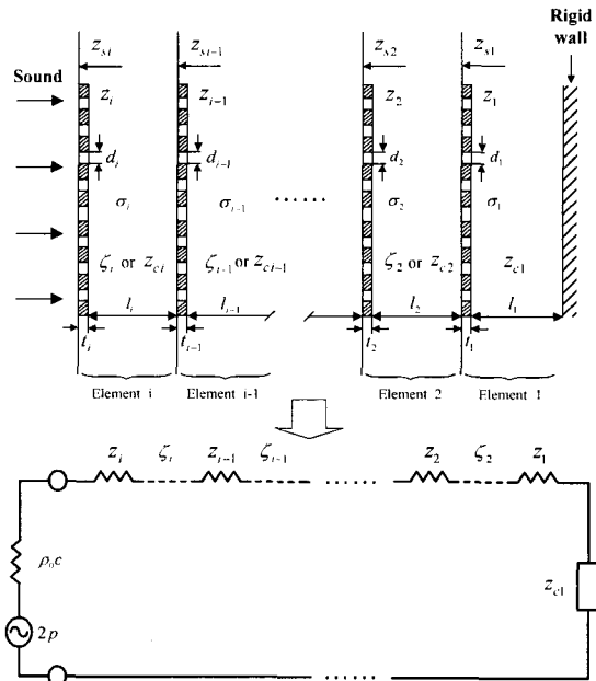
Fig. 2 Multiple layer perforated plate system and equivalent electroacoustic circuit by treating the airtspaces between perforated plates as distributed elements
