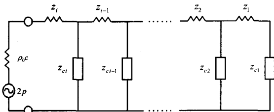
Fig. 3 Equivalent electroacoustic circuit by regarding airspaces between perforated plates as shunt lumped elements like the previous works
