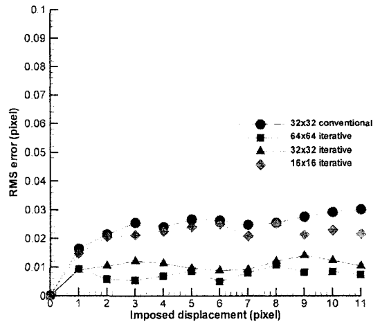
Fig. 5 Measurement RMS error as a function of particle displacement
