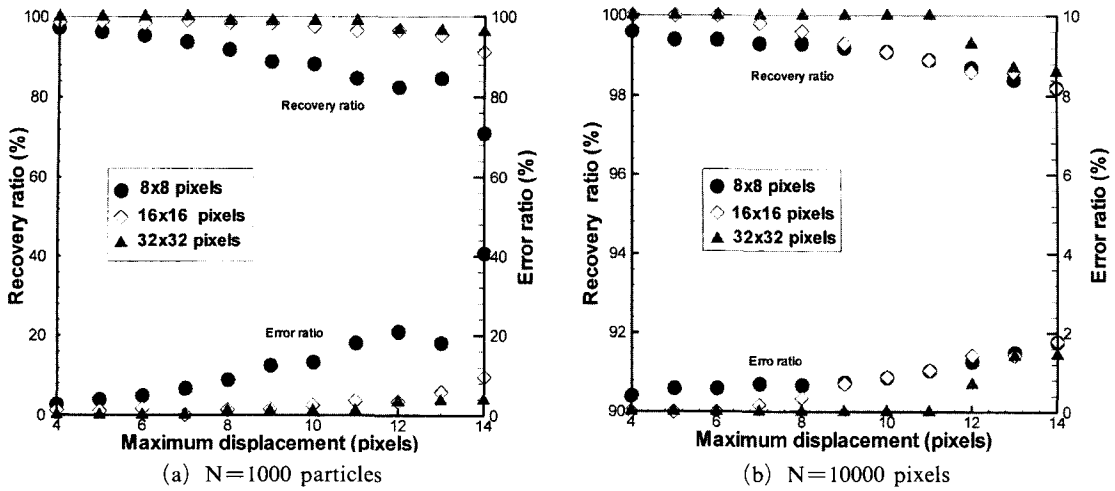
Fig. 6 Recovery/errro ratio vs. maximum displacement for solid body rotation, image size : 256 \times 256 pixels
