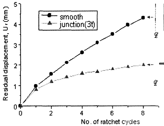
Fig. 12 Comparison of test results for smooth cylinder and cylinder with plate-to-shell junction
