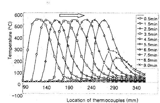
Fig. 7 Temperature profiles measured by 28 channel thermocouples
