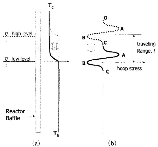
Fig. 2 Concept of moving temperature front and corresponding hoop stress distribution
