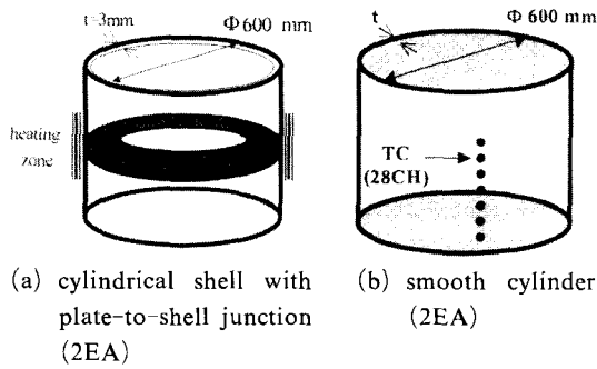
Fig. 6 Schematic diagram of the test cylinders
