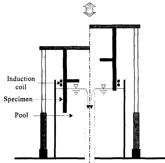
Fig. 4 Schematic diagram of thermal ratcheting test facility
