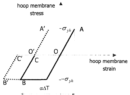
Fig. 3 Stress-strain loci in shrinkage region
