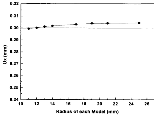
Fig. 6 Horizontal displacement of valve tip with respect to the variation of radius of curvature in model of type II
