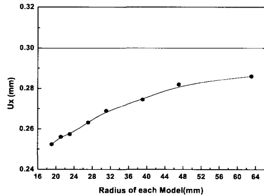
Fig. 8 Horizontal displacement of valve tip with respect to the variation of radius of curvature in model of type III
