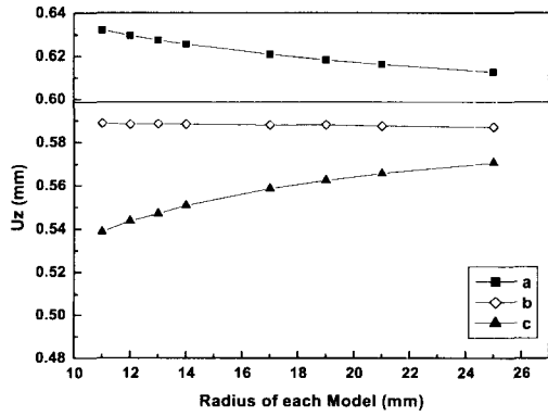
Fig. 5 Maximum vertical displacement of each region with respect to the variation of radius of curvature in model of type II
