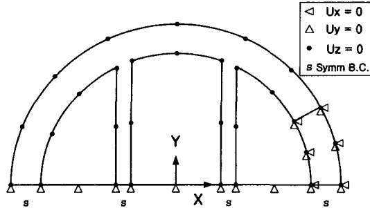
Fig. 3 Boundary condition of model
