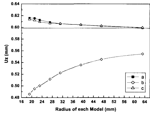
Fig. 7 Maximum vertical displacement of each region with respect to the variation of radius of curvature in model of type III
