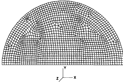
Fig. 4(a) The mesh of valve in model type II
