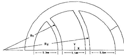
Fig. 2(a) The shape of model type II
