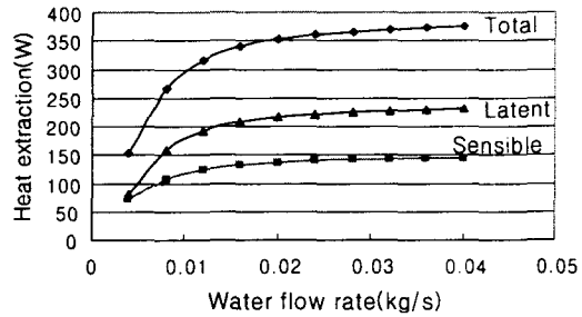
(a) Case 1. Water flow rate adjustment
