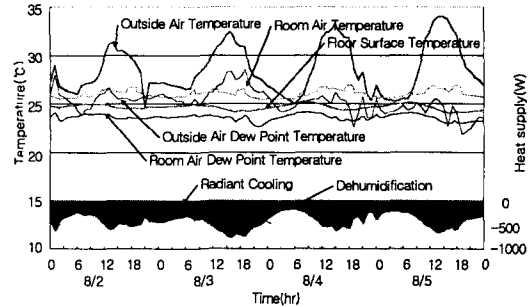
(a) Case 1. Water flow rate adjustment
