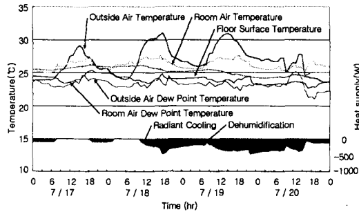
(a) Case 1. Water flow rate adjustment
