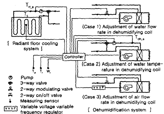
Fig. 2 Schematic diagram of control methods in integrated system.
