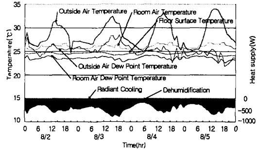
(b) Case 2. Water temperature adjustment
