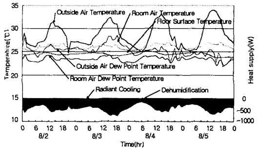
(c) Case 3. Air flow rate adjustment
