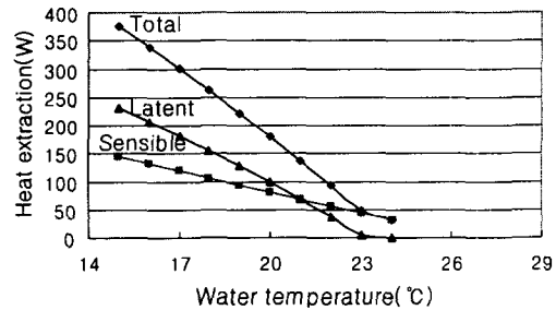
(b) Case 2. Water temperature adjustment
