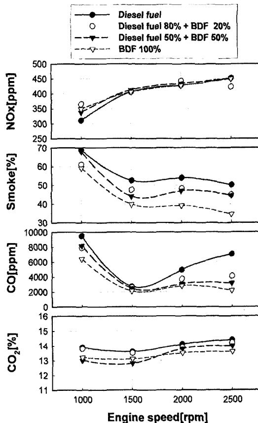
Fig. 5 Exhaust emissions versus engine speed at engine load 100%
