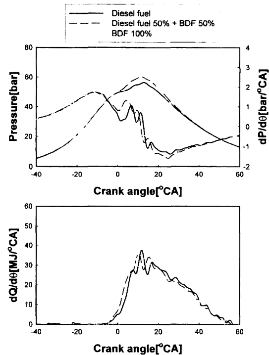
Fig. 3 Pressure, dP/d\theta , and dQ/d\theta at engine speed 2500 rpm and load 100%
