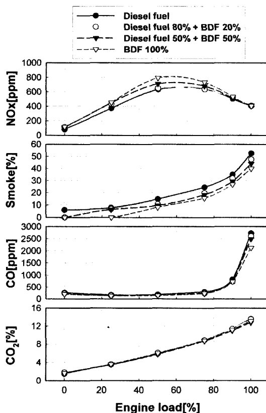
Fig. 7 Exhaust emissions and BSEC versus engine load at engine speed 1500 rpm
