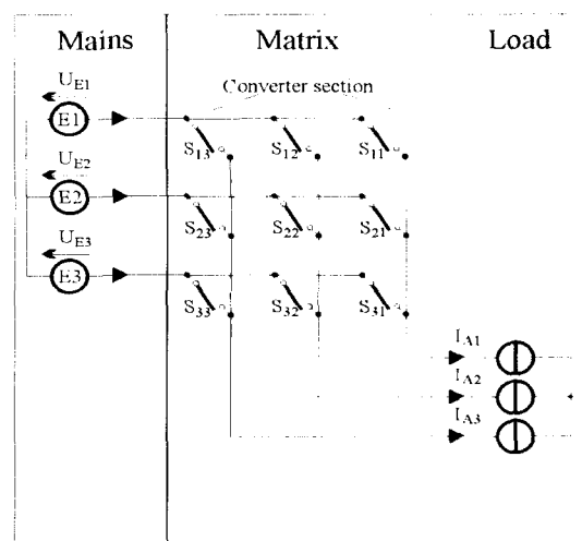
Fig. 1. Ideal 3x3 matrix converter technology.
