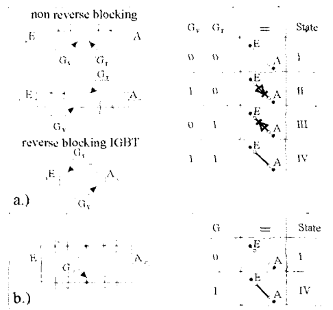
Fig. 3. Discrete structure of bi-directional switches.
