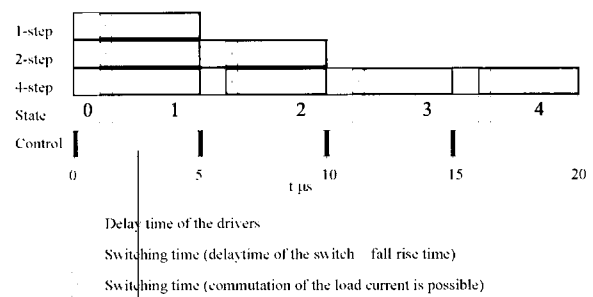
Fig. 7. Float diagram of multi stepped commutation policies.
