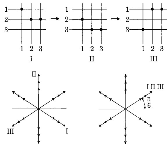
Fig. 9. Switching states and pulsating vectors.
