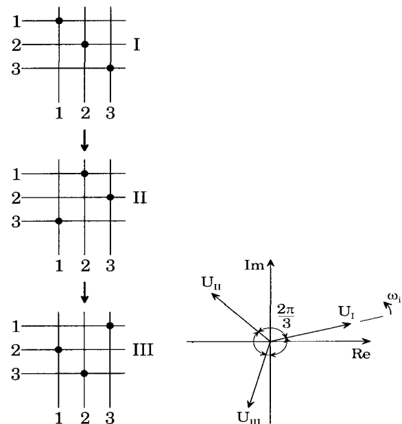
Fig. 10. Switching states and left rotating vectors.
