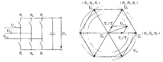
Fig. 12. Space vector modulation for front-end converter.
