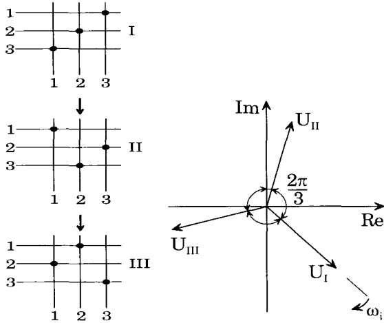
Fig. 11. Switching states and right rotating vectors.
