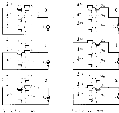
Fig. 5. Two steps commutation.
