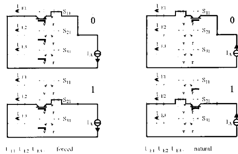
Fig. 6. One step commutation.
