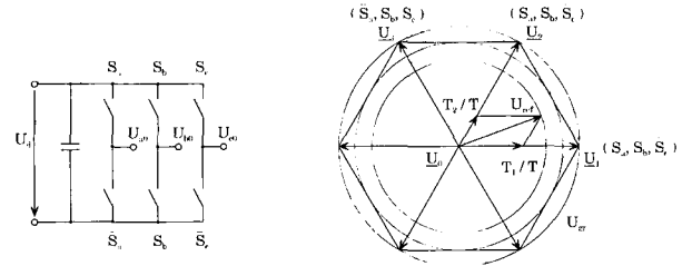
Fig. 13. Space vector modulation for inverter.
