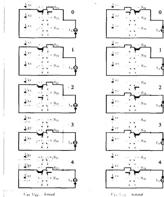
Fig. 4. 4 steps commutation of load current phase 1 to phase 2 without using switches of phase 3; I detection; U don't care.
