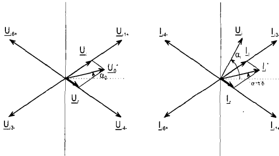
Fig. 14. Space vector modulation for matrix converters.
