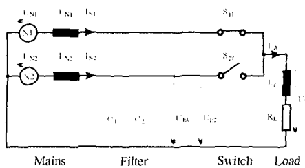
Fig. 2. Commutation problem.
