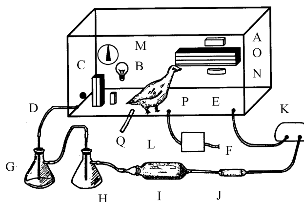
Figure 1. The respiration chamber and accessory equipment. A, fan, B, light globe, C, sample outlet, D, circulation outlet, E, circulation inlet, F, connected to oxygen tank, G, water trap (with desiccant), H, flask containing KOH, I, Water trap, J, filtration train, K, pump, L, timer and pressure valve, M, thermometer, N, hygrometer, O, radiator, P, inlet for oxygen, Q, power supply.
