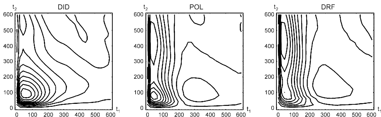
Figure 2. The \chi_{mzzzz}^{(5)} two-dimensional Raman response in the DID, POL and DRF models, where m denotes the magic angle compared to the z -axis. The time is given in fs.
