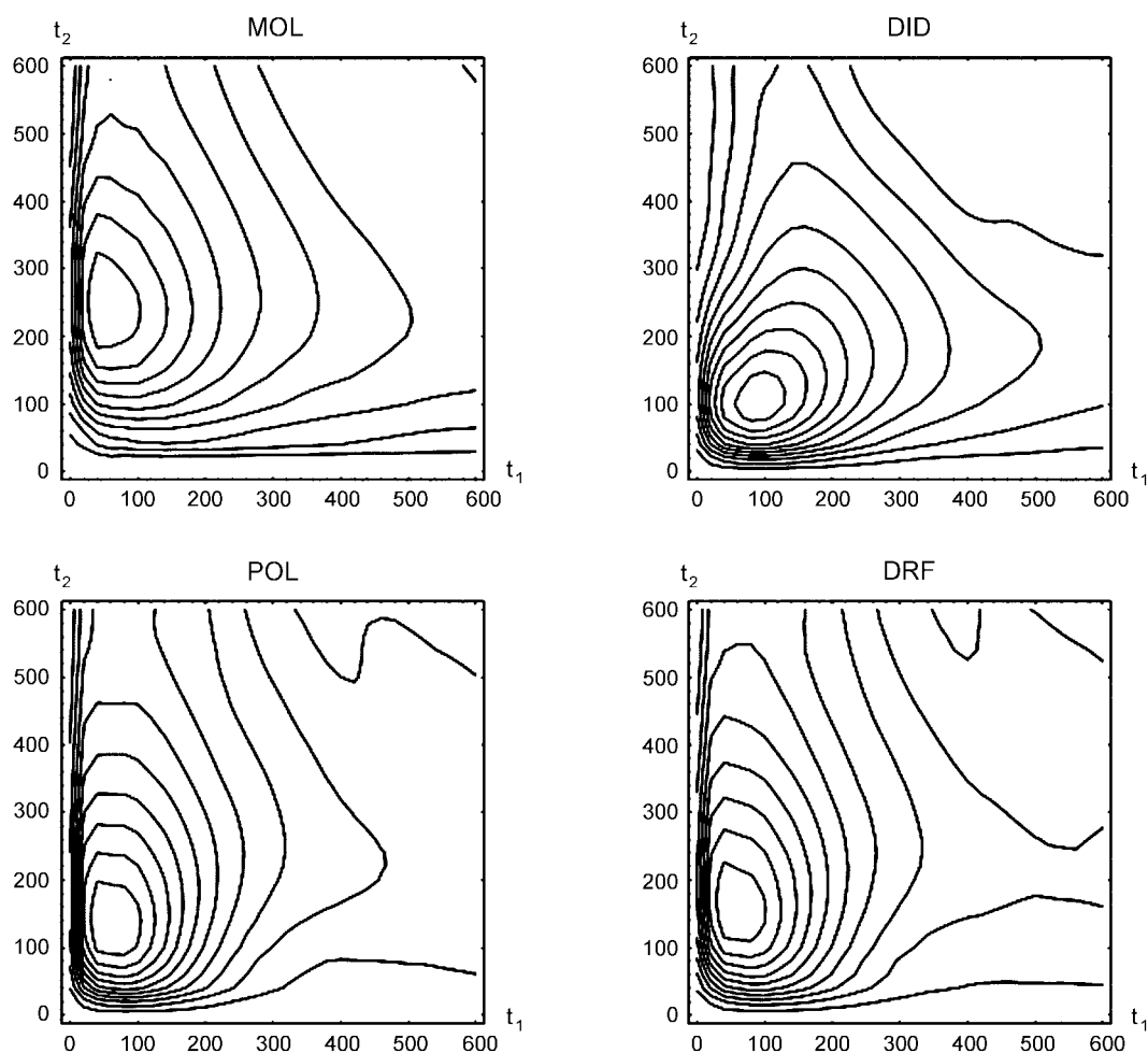
Figure 1. The all polarized two-dimensional Raman response \chi_{\text{isotropic}}^{(5)} in the MOL, POL, DID and DRF models. The time is given in fs.
