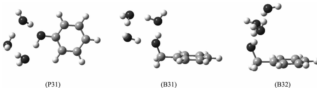
Figure 4. Structures of lowest-energy phenol- and benzyl alcohol-(H 2 O) 3 clusters.
