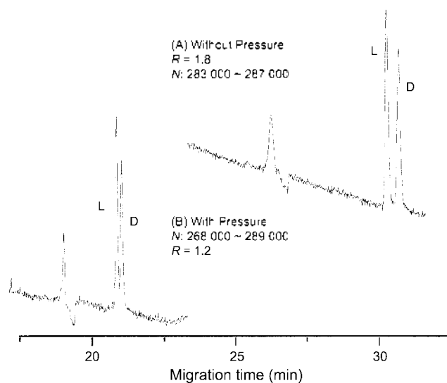
Figure 2. MEKC electropherograms demonstrating the pressure effect in MEKC-UV system. (A) Applied voltage of 28.4 kV without pressure at 25 ^{\circ} C. (B) Applying voltage of 28.4 kV and low pressure of 0.5 psi at 25 ^{\circ} C. Others MEKC conditions: running buffer, 20 mM ammonium acetate buffer (pH 7.0) and 30 mM SDS; a bare fused-silica capillary of 127 cm long (effective length 120 cm) \times 50 \mu m i.d.; hydrodynamic injection for 5 s at 0.5 psi. Sample: 100 \mu g/mL D-amygdalin dissolving in solution of pH 11.0. *Indicates: N = Efficiency, R = Resolution.
