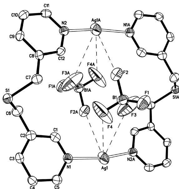
Figure 1. Structure of complex [\text{Ag}(\text{I})]_2 \cdot 2\text{BF}_4 with atomic labeling scheme. Hydrogen atoms are omitted for clarity.
