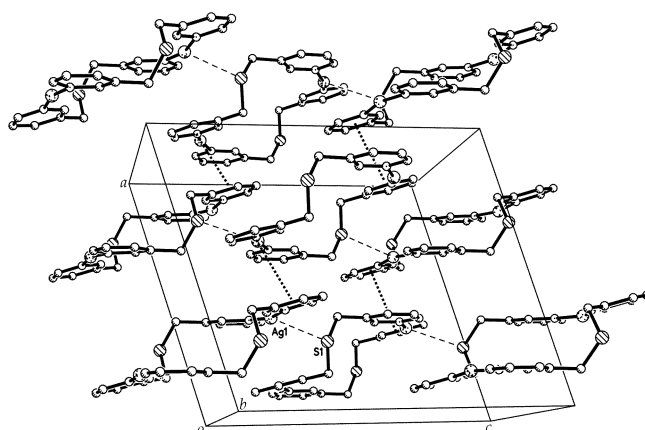
Figure 2. Projection showing the stair-shaped cyclic dimers with the Ag...S and \pi - \pi interactions for [\text{Ag}(\text{I})]_2 \cdot 2\text{BF}_4 . \text{BF}_4^- ions and H atoms are omitted for clarity.
