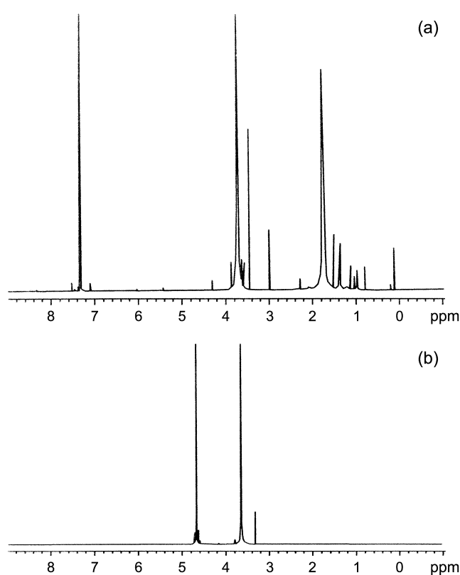
Figure 2. 1 H-NMR spectra of LMWSC-NP in CDCl 3 (a) and D 2 O (b)
