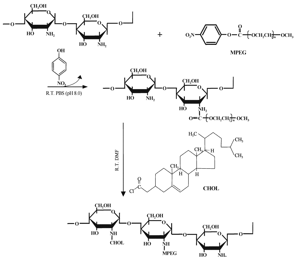
Scheme 1. Synthetic route of LMWSC-NPs.
