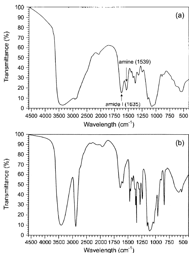
Figure 1. FT-IR spectra of LMWSC (a) and LMWSC-MPEG (b).
