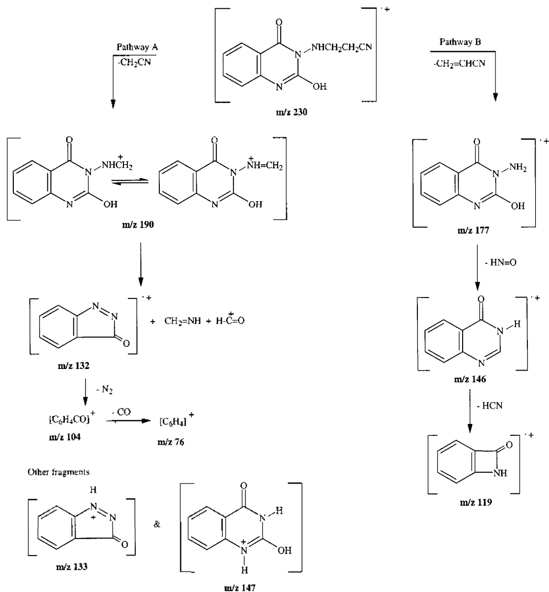
Scheme 6. Main fragmentation pathway of compound 6a , as a representative example for compounds 5 , and 6a, b .
