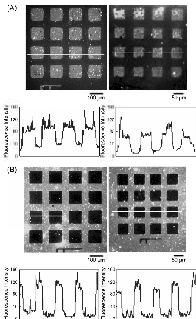
Figure 2. Fluorescence images of the dendrimer-printed gold surface incubated with fluorescent microbeads. Positive (A) and negative (B) patterns with the feature sizes of 100\ \mu\text{m} and 50\ \mu\text{m} are shown with scale bars. Also shown are fluorescence profiles across the white lines drawn on images.
