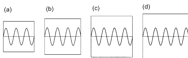
Figure 1. The relationship between the thermal wavelength and the molecular free space. The nodes of thermal wavelength lie on the boundary of molecular free space, resulting in stationary wave functions. (a) 15 °C ( q = 3.0 ), (b) 30 °C ( q = 3.5 ), (c) 45 °C ( q = 4.0 ), and (d) 60 °C ( q = 4.5 ). These quantum number arise for heavy water are at 19, 32, 44, 56 °C, respectively. The same phenomena are at the melting point ( q = 2.5 ), and at -16 ( q = 2.0 ) and -36 °C ( q = 1.5 ) in the supercooled region.
