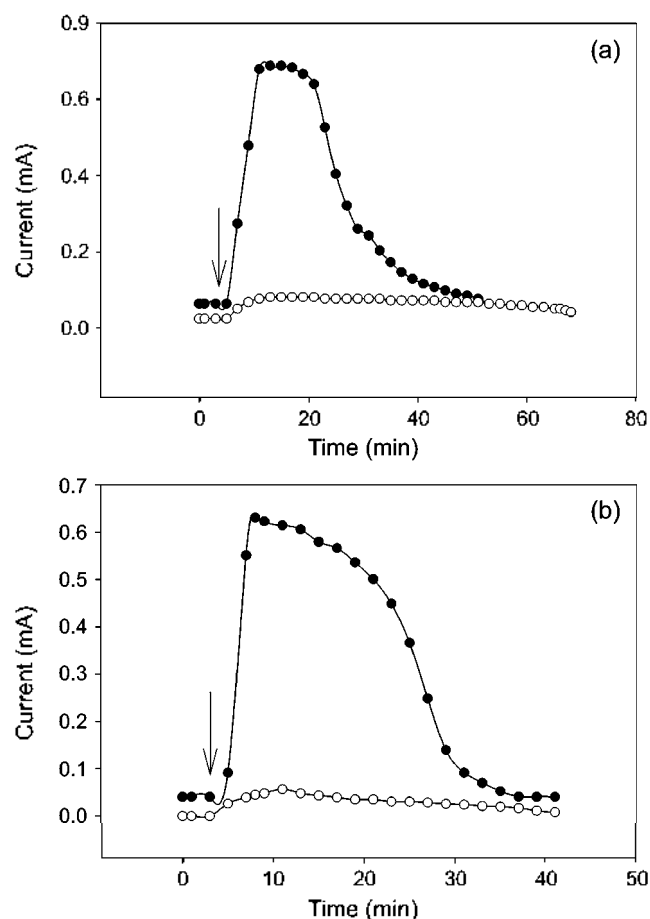
Figure 1. Variation of current output with time through the 560- \Omega external load for fuel cells containing (a) P. vulgaris and (b) E. coli with safranin O (○) and thionin (●) as the electron transfer mediator. Organism concentration: 1 mg (dry wt) mL -1 ; 1 \mu\text{mol} of mediator and 1 \mu\text{mol} of glucose were added. Addition of glucose is marked by the arrows.
