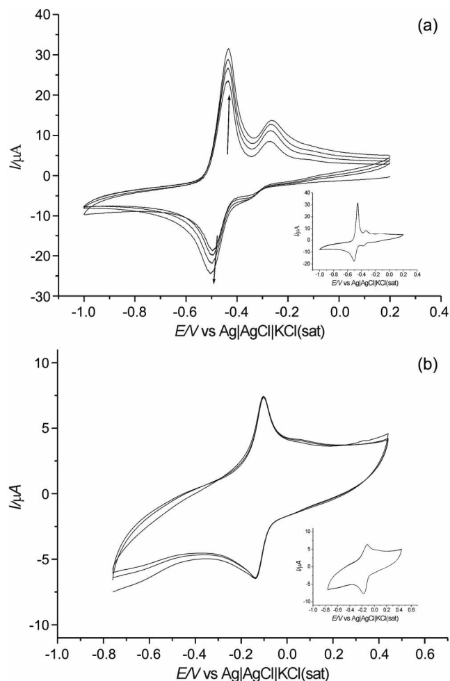
Figure 2. Cyclic voltammograms of safranin O (a) and thionin (b) in the PC film at pH 7.0 solution. Scan rate: 100 \text{ mV s}^{-1} . Electrode area: 0.071 \text{ cm}^2 . Inset shows the voltammogram on the bare electrode.
