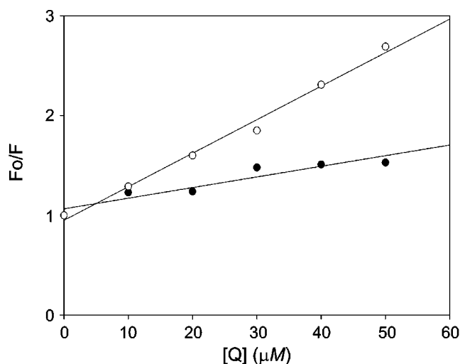
Figure 3. Plot of F_0/F vs [Q] according to Stern-Volmer equation in aqueous medium with safranin O (○) and thionin (●). Calculated Stern-Volmer quenching constants ( K_{SV} ) of mediators are 0.0336 \text{ M}^{-1} for safranin O and 0.0107 \text{ M}^{-1} for thionin.
