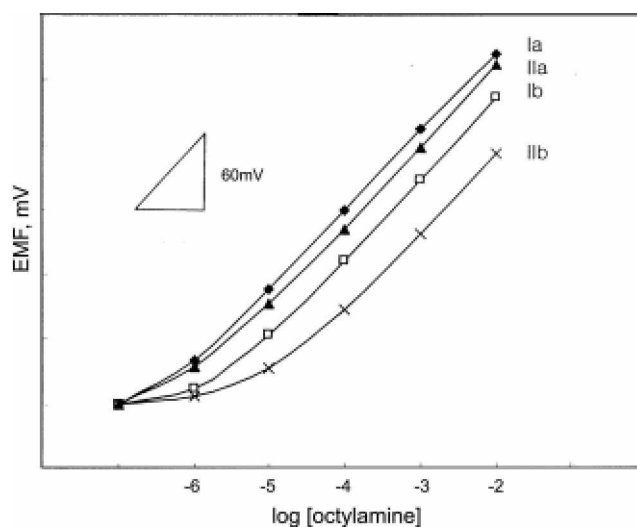
Figure 4. The potentiometric response curves of electrodes No. 1-4 to the concentration change of octylamine in pH 7.2 buffer solution.
