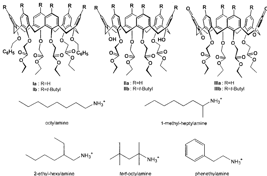
Figure 1. Six lipophilic tetraesters of calix[6]arene ( Ia-IIIb ), calix[6]diquinone ( IIIa, IIIb ), and the organic amine guests.
