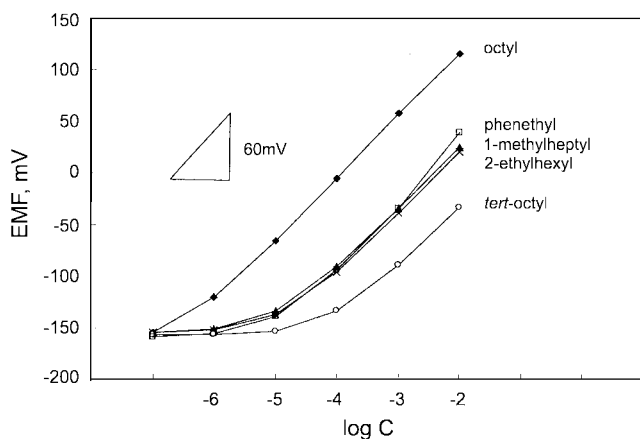
Figure 3. The potentiometric response curves of the electrode No. 1 based on calix[6]arene tetraester Ia to the concentration change of amine guests in pH 7.2 buffer solution.
