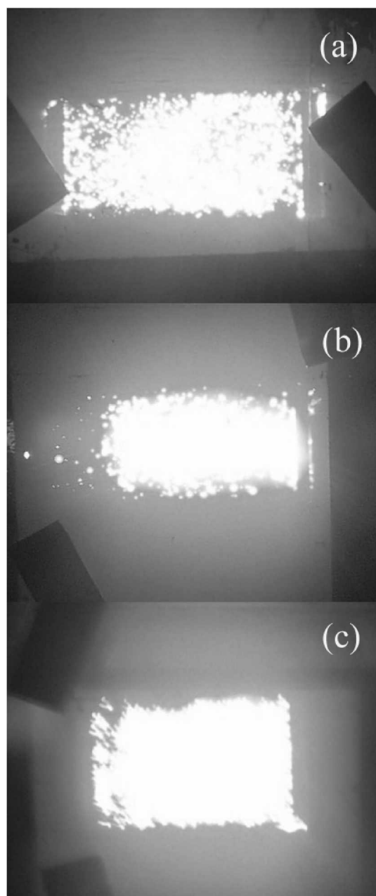
Figure 5. Emission patterns of the CNTs fabricated by CO disproportionation at (a) 500, (b) 550, (c) 600 °C by applying 4.0, 3.4 and 3.1 V/μm, respectively.
