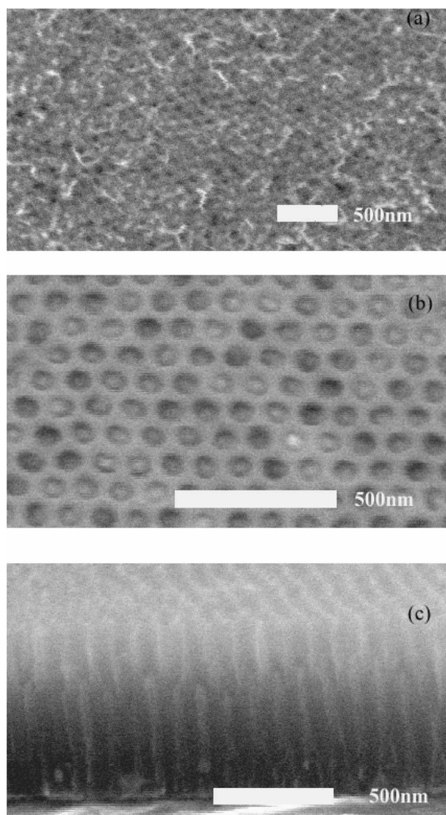
Figure 1. SEM images of an AAO template deposited Co: (a) the surface view after deposition of Co, and (b) the surface and (c) a cross-sectional views after being treated with H_2SO_4 and then NaOH solutions. Co is about 160 nm below the surface in the pores after etching in acid and base solutions.
