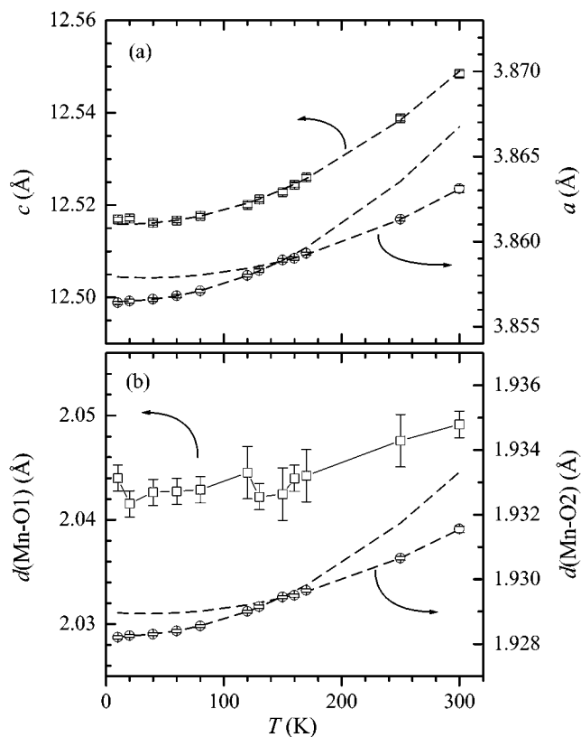
Figure 1. (a) Temperature dependence of lattice parameters of a (open circle) and c (open rectangle) and (b) Variations of the Mn-O1 (open rectangle) and Mn-O2 (open circle) bond lengths for La 1-x -Sr 1-3 MnO 4+δ . Dashed lines are fitting curves.
