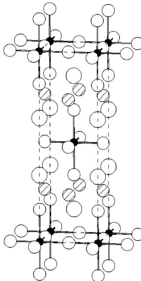
Figure 2. Structure of La 1-x -Sr 1-3 MnO 4+δ . Large open circles, small open circles and hatched circles represent La/Sr atoms, oxygen atoms and interstitial oxygen O3 atoms, respectively.
