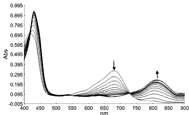
Figure 1. UV-Vis. Spectral titration with tetrabutylammonium fluoride (TBAF). [2] = 2.65 \times 10^{-5} M in \text{CHCl}_3 at 25 °C. Each spectrum was taken after adding 0.1 equiv. of guest.
