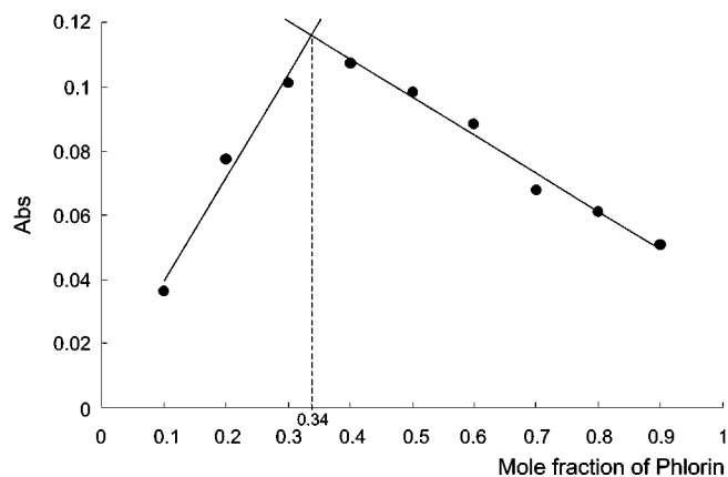
Figure 2. Job plot for 2 with TBAF, [2] = 4.2 \times 10^{-5} M in \text{CHCl}_3 at 25 °C.
