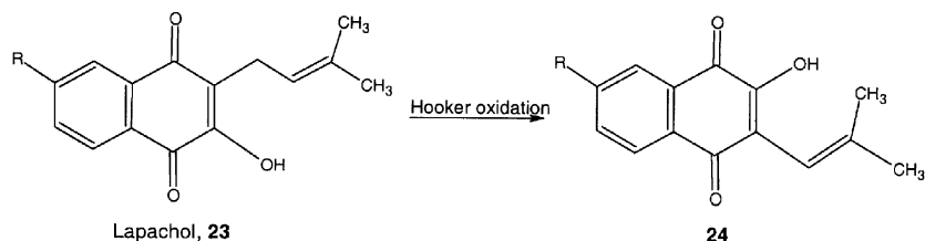
Scheme 7. Hooker oxidation.
