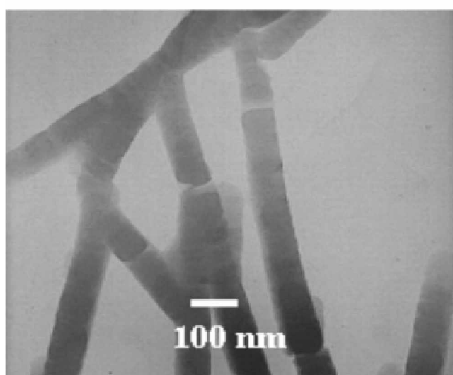
Figure 3. TEM pictures of magnetically aligned cobalt nanoparticles. Cobalt nanoparticles (synthetic condition: micelle concentration = 0.3 and water content = 40 \mu L) were magnetically aligned by slow oxidation with O_2 under the external magnetic field.
