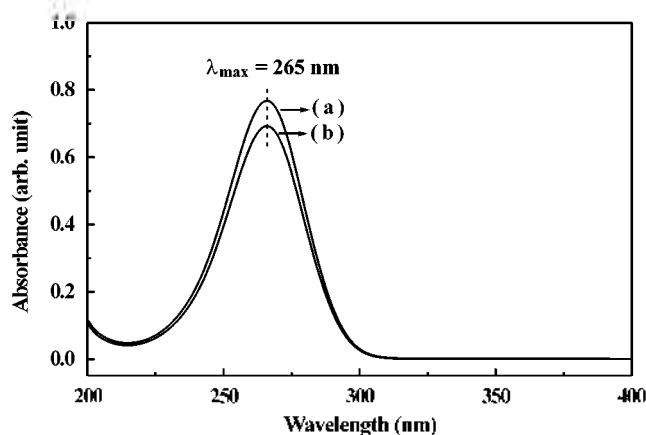
Figure 4. UV-vis spectra of (a) released vitamin C from Vitabrid-C and (b) pure vitamin C (sodium L-ascorbate).
