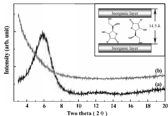
Figure 1. Powder X-ray diffraction patterns of (a) vitamin C-hydrated zinc oxide nanohybrid and (b) Vitabrid-C, respectively.
