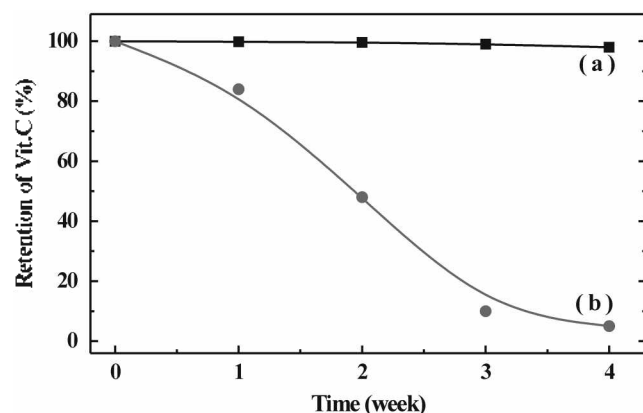
Figure 5. Retention of vitamin C in (a) Vitabrid-C and (b) pure vitamin C (sodium L-ascorbate) at 42 °C in aqueous medium.
