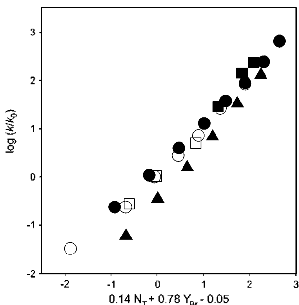
Figure 2. Plot of \log(k/k_0) for cinnamyl bromide against (0.14N_T + 0.78Y_{Br} - 0.05) ; r = 0.980 (solvent codes: ●, methanol; ○, ethanol; ▲, acetone; ■, TFE-H 2 O; □, TFE-EtOH).
