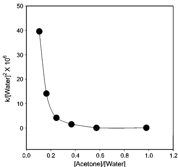
Figure 4. Plot of third-order rate constant versus [\text{Acetone}]/[\text{Water}] .
