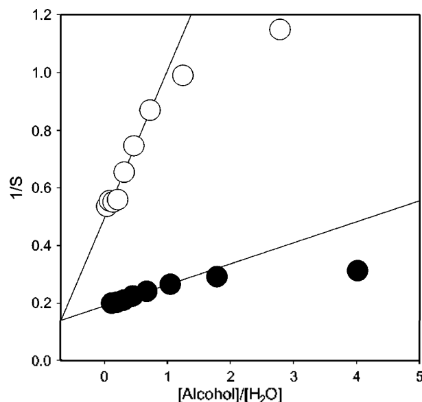
Figure 5. Plot of 1/S vs. molar ratio of solvents versus [\text{alcohol}]/[\text{water}] , for solvolysis of cinnamyl bromide at 25 (solvent codes: ●, methanol; ○, ethanol) (ethanol: slope = 0.513, intercept = 0.497; methanol: slope = 0.00924, intercept = 0.276).
