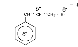
Scheme 2. Proposed Transition State Structure.
