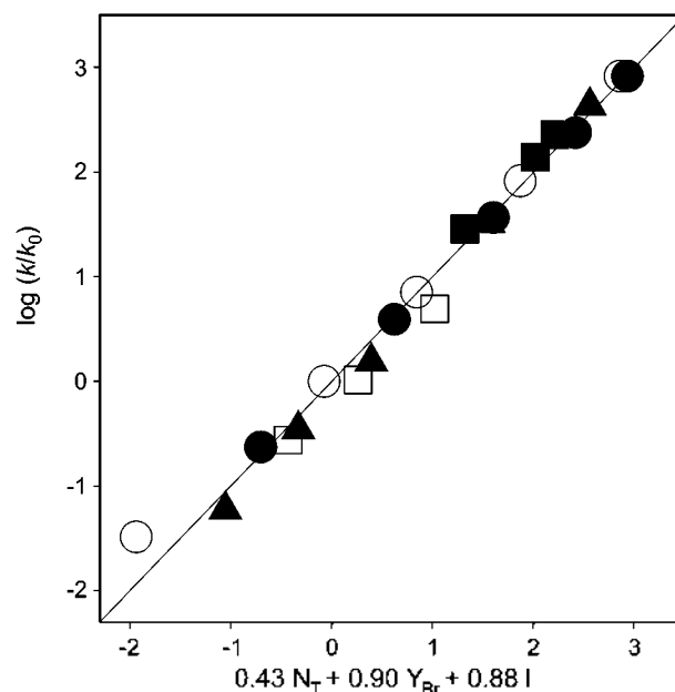
Figure 3. Plot of \log(k/k_0) for cinnamyl bromide against (0.43N_T + 0.90Y_{Br} + 0.88l) ; r = 0.995 (solvent codes: ●, methanol; ○, ethanol; ▲, acetone; ■, TFE-H 2 O; □, TFE-EtOH).
