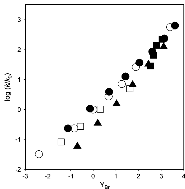
Figure 1. Logarithms of first-order rate constants for solvolysis of cinnamyl bromide at 25 °C: \log(k/k_0) vs. Y_{Br} (solvent code: ●, methanol; ○, ethanol; ▲, acetone; ■, TFE-H 2 O; □, TFE-EtOH).
