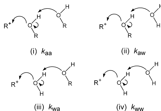
Scheme 1. General base catalyzed reactions for nucleophilic attack on carbocations.
