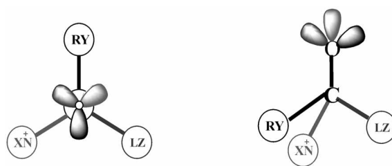
Figure 2. Antiperiplanar lone pairs on the oxygen atom to the three bonds, C-N^+X , C-LZ and C-RY , in a zwitterionic tetrahedral intermediate, T^\ddagger .
