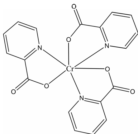
Scheme 1. Structure of chromium(III) picolinate (Cr-(pic) 3 ).
