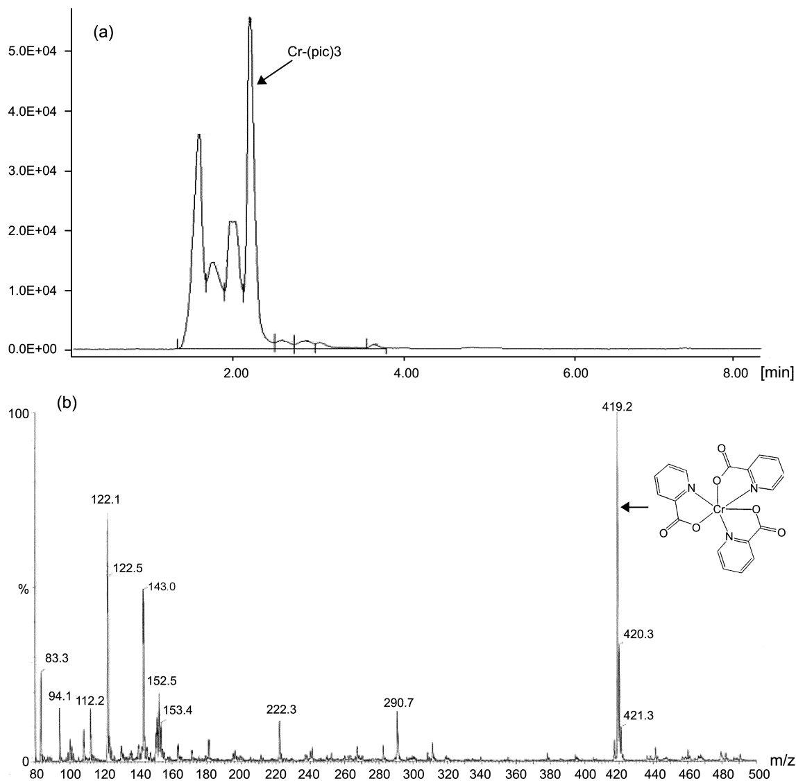
Figure 4. (a) Chromatogram obtained from feed product (company C); same conditions as described in Figure 1(b) the ESI mass spectrum detected directly after I.C separation (peak time = 2.15 min), peak; 419 m/z [M·H].
