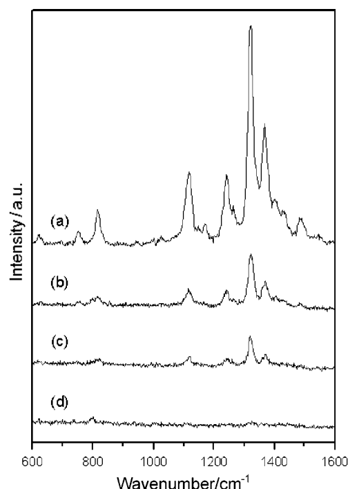
Figure 8. SERS spectra of different concentrated quinomethionate: (a) 10^{-3} M (b) 10^{-4} M (c) 10^{-5} M (d) 10^{-6} M.
