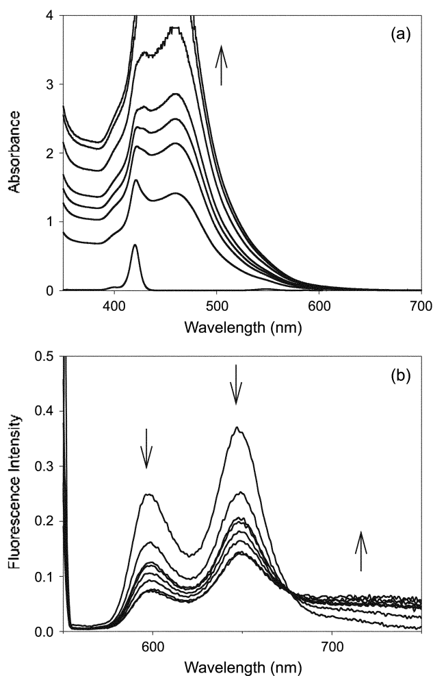
Figure 4. Absorption (a) and fluorescence (b) spectral changes of ZnTTP in dichloromethane on the addition of Ru(bpy) 2 (mbpy~py)(PF 6 ) 2 : [ZnTTP] = 1.0 × 10 -6 M, [Ru(bpy) 2 (mbpy~py)(PF 6 ) 2 ] = 0, 8.0 × 10 -5 , 1.2 × 10 -4 , 1.4 × 10 -4 , 1.6 × 10 -4 , 2.0 × 10 -4 , 2.6 × 10 -4 , 2.8 × 10 -4 M.
