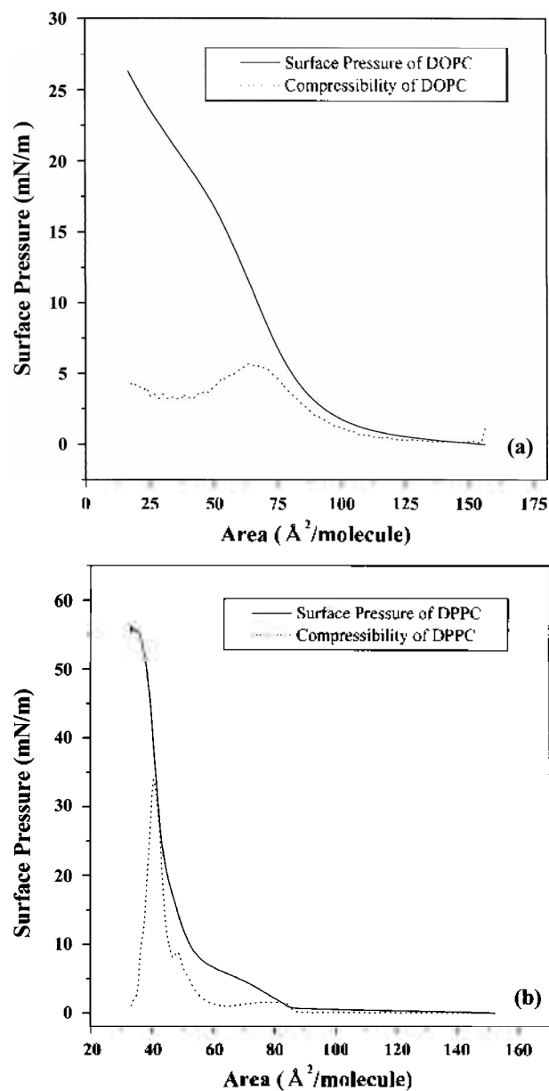
Figure 5. The \pi -A isotherms (—) and compressibility (---) of (a) DOPC(C8) and (b) DPPC(C16) at 20 °C.
