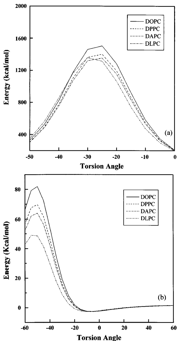
Figure 6. (a) Conformational energy curves of DOPC(C8), DPPC(C16), DAPC(C20), and DLPC(C24), (b) Interaction energy curve between two ( \beta , \gamma ) chains of DOPC(C8), DPPC(C16), DAPC(C20), and DLPC(C24) by CHARMM lipid force field.
