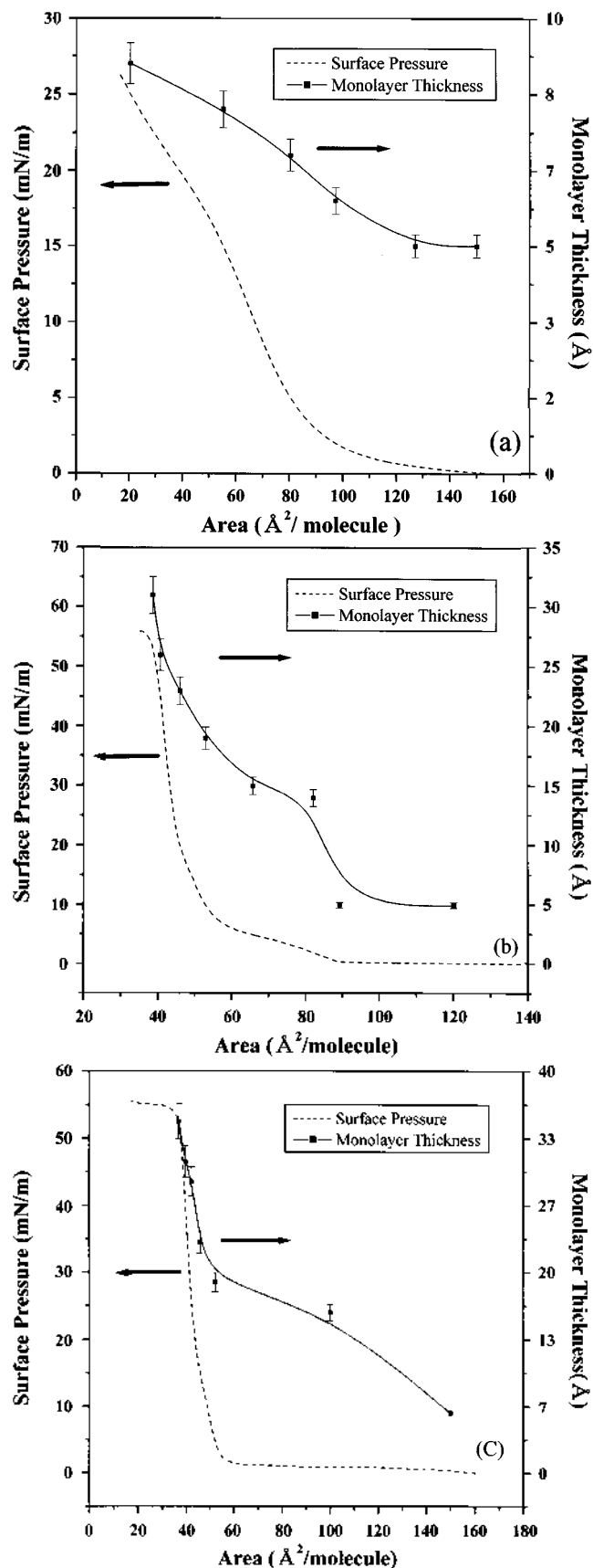
Figure 3. The \pi -A isotherms (—) and monolayer thickness vs. area per molecule ( A_m ) curves (■) of (a) DOPC(C8), (b) DPPC(C16), and (c) DLPC(C24), at the air-water interface. The monolayer thickness was measured by ellipsometer.
