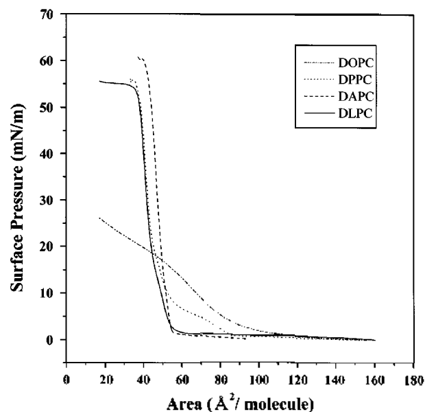
Figure 2. The \pi -A isotherms of PCs with different alkyl chain lengths, DOPC(C8), DPPC(C16), DAPC(C20), and DLPC(C24), at 25 °C.
