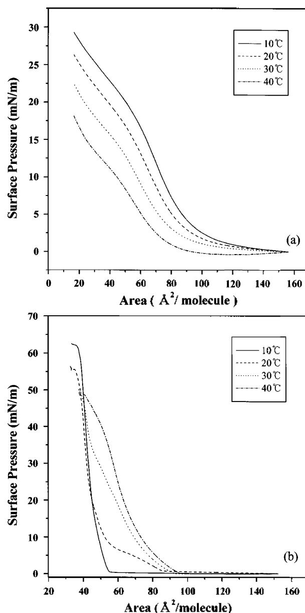
Figure 4. The \pi -A isotherms of (a) DOPC(C8), (b) DPPC(C16), (c) DAPC(C20), (d) DLPC(C24), and (e) POPC with various temperatures at the air/water interface.
