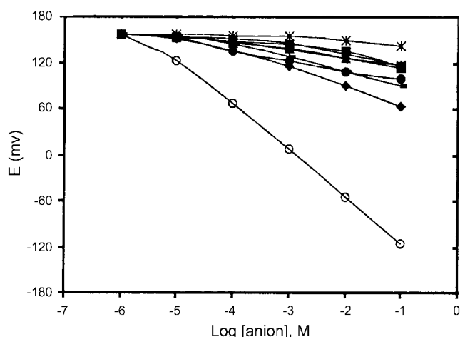
Figure 2. Potential responses of different ionselective electrodes based on titanium. Acetylacetonate: (●) Cyanide, (■) Nitrate, (▲) Nitrite, (◆) Thiocyanate, (⊕) Acetate, (⊕) Chloride, (⊖) Iodide, (⊖) Bromide, (⊖) Perchlorate, (⊖) Salicylate).
