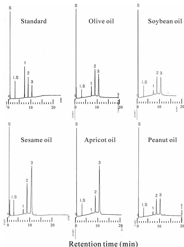
Figure 1. Separation of intact triacylglycerols in selected vegetable oils by high temperature gas chromatography with flame ionization detector. (S: solvent, I.S.: internal standard ( T_{52} ), 1: T_{50} , 2: T_{52} , 3: T_{54} )
