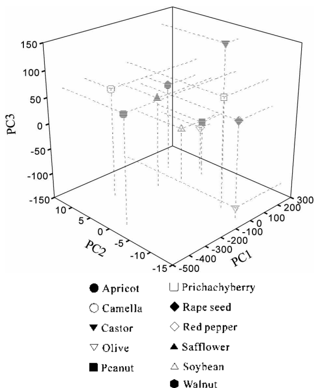
Figure 2. Principal components plot for intact triacylglycerols composition of selected vegetable oils listed in Table 1.
