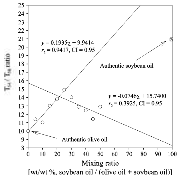
Figure 3. Relationship of mixing ratio of soybean oil in olive oil and relative ratio of T_{54}/T_{50} .
