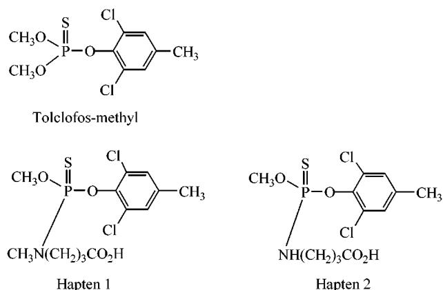
Figure 1. Structures of the haptens for tolclofos-methyl used for immunization (Hapten 1), antigen coating (Hapten 2) and enzyme tracer (Hapten 2).
