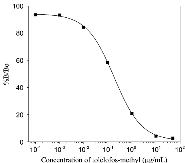
Figure 3. Standard curve for tolclofos-methyl by competitive indirect ELISA using the antiserum against Hapten 1-BSA diluted 1/2000, the coating antigen Hapten 2-OVA (15 ng/well) and gelatin blocking agent (1%). The composition of the assay solution was 10% methanol-PBS (100 mM).
