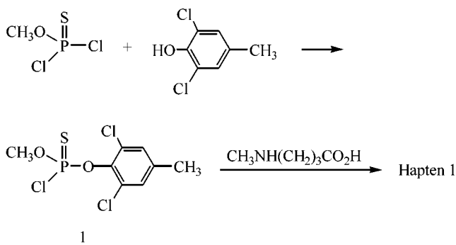
Figure 2. Synthetic route for Hapten 1.
