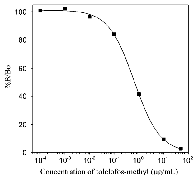
Figure 4. Standard curve for tolclofos-methyl by competitive direct ELISA using the antiserum against Hapten 1-BSA diluted 1/1000, the enzyme tracer Hapten 2-HRP and gelatin blocking agent (1%).
