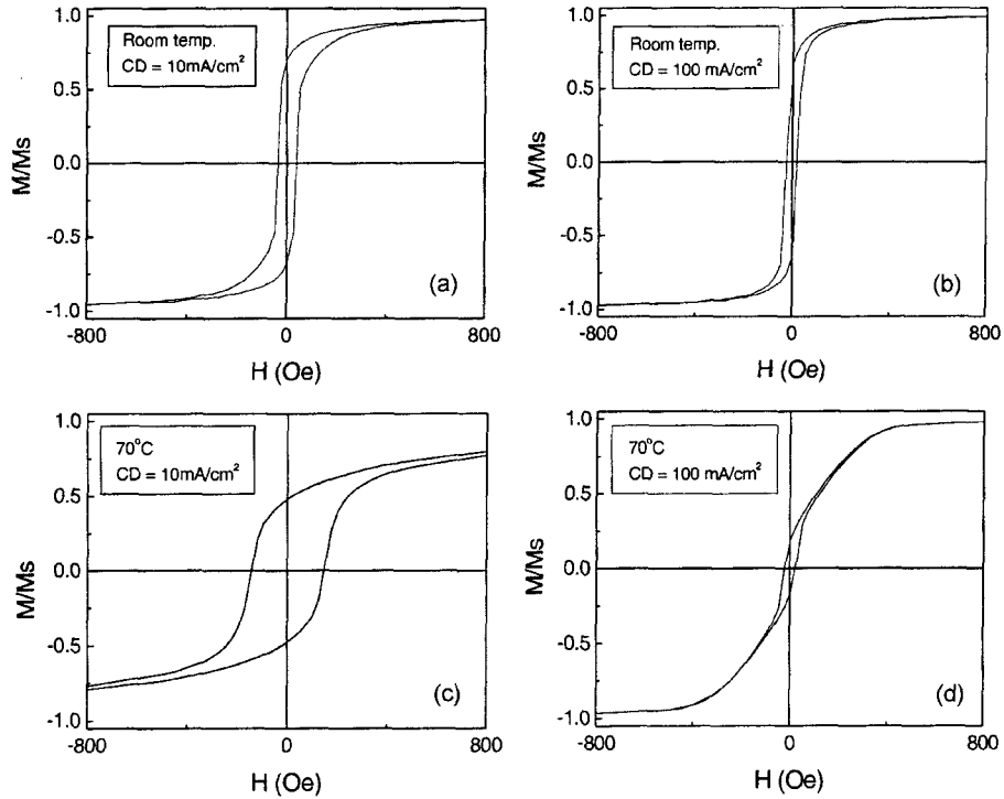
Fig. 6. Dependence of parallel B-H loop of the CoW thin film alloys electrodeposited at room temperature and 70°C on current density.
