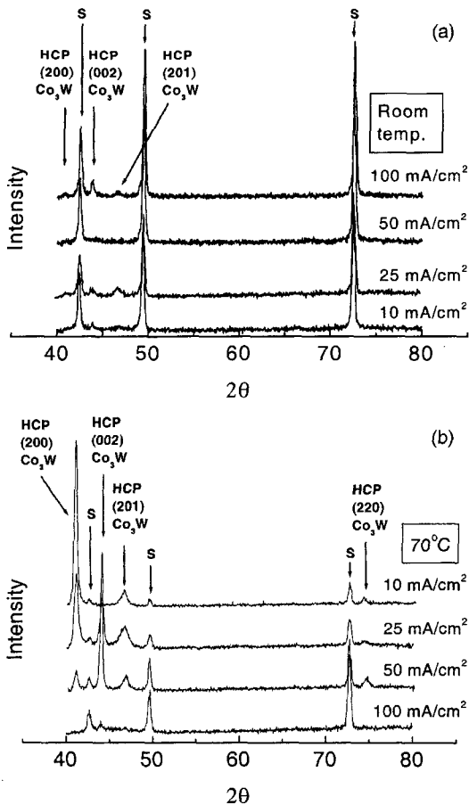
Fig. 7. XRD patterns of CoW thin film electrodeposited with various current densities at (a) room temperature and (b) 70°C.
