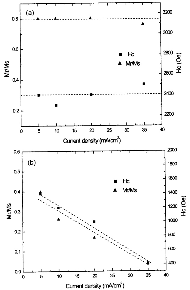
Fig. 3. Variation of magnetic properties depending on the current density. Results are given for CoP nanowires with the diameter of 20 nm (a) and 200 nm (b), respectively.
