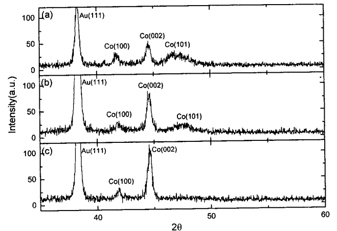
Fig. 4. X-ray diffraction patterns of CoP disk film according to the current densities; 35 mA/cm 2 (a), 15 mA/cm 2 (b), and 5 mA/cm 2 (c).
