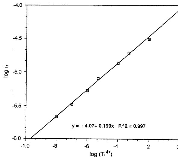
Fig. 7. Calibration curve for determination of Ti^{4+} ions originated from Fig. 6.
