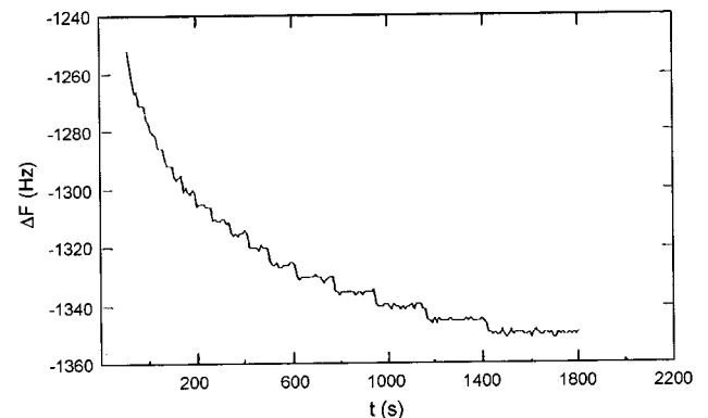
Fig. 4. Frequency response to time for QCA(Au)/p-3,4-DHBA electrode in 0.1 M phosphate buffer solution (pH = 7.07) containing 1 mM dopamine.
