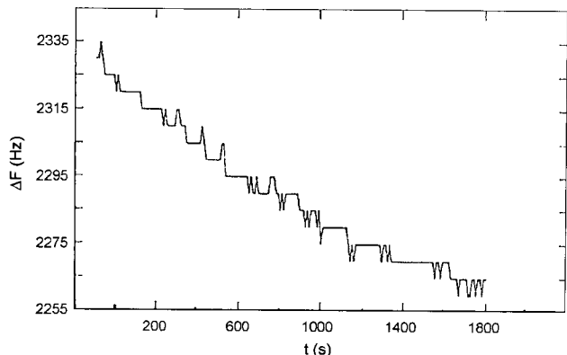
Fig. 5. Frequency response to time for QCA(Au)/p-3,4-DHBA-dopa electrode in 0.1 M phosphate buffer solution (pH = 7.07) containing 1.05 \times 10^{-4} M Ti^{4+} .
