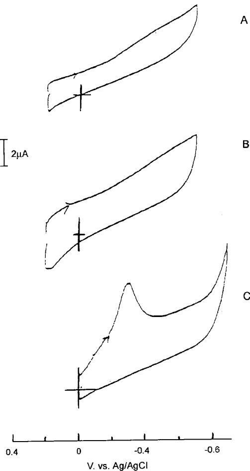
Fig. 2. Cyclic voltammograms of the electrode type of GC/p-3,4-DHBA: (A), GC/p-3,4-DHBA-dopa: (B) and GC/p-3,4-DHBA-dopa ( Ti^{4+} ): (C) at potential range of 0.2 to 0.7 V in 0.1 M phosphate buffer (pH = 7.07); (scan rate: 0.05 V/s, electrode area: 3.15 \times 10^{-2} \text{ cm}^2 )
